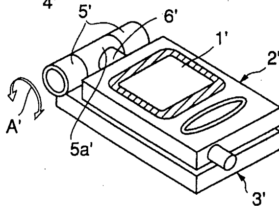
FIG.2C (PRIOR ART)
