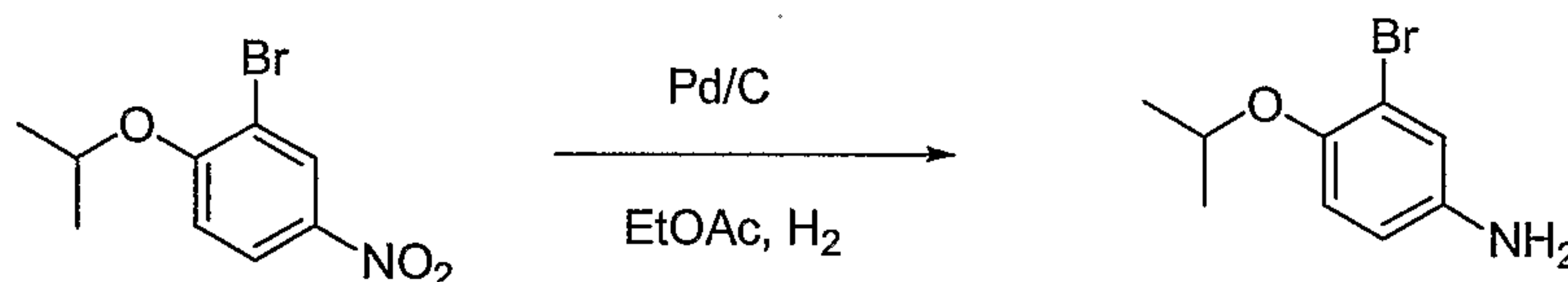
3-Bromo-4-isopropoxy-phenylamine
