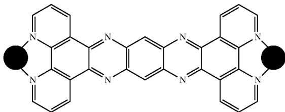
Scheme 1B.
