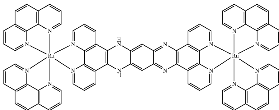
Scheme 6.
