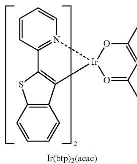
Ir(btp) 2 (acac)
