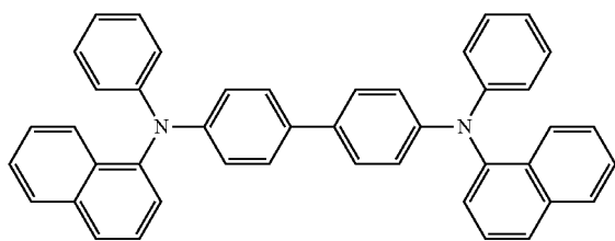
NPD
