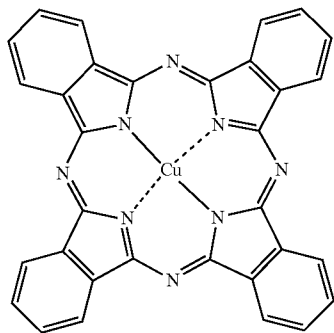
CuPC
