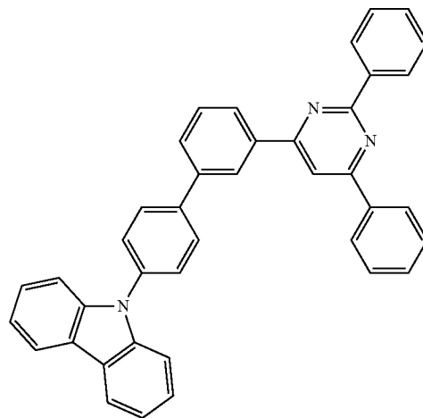
Ir(btp) 2 (acac)
