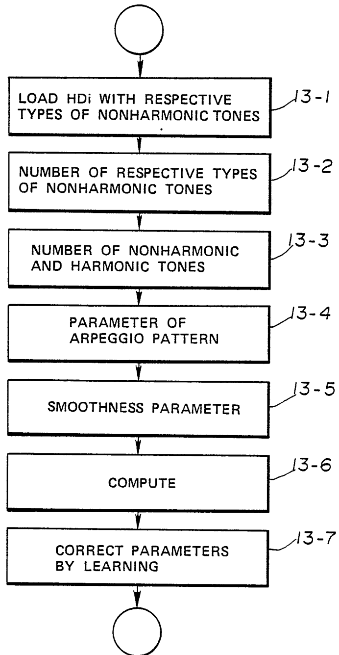
FIG.13 EXTRACT AND COMPUTE PARAMETERS
