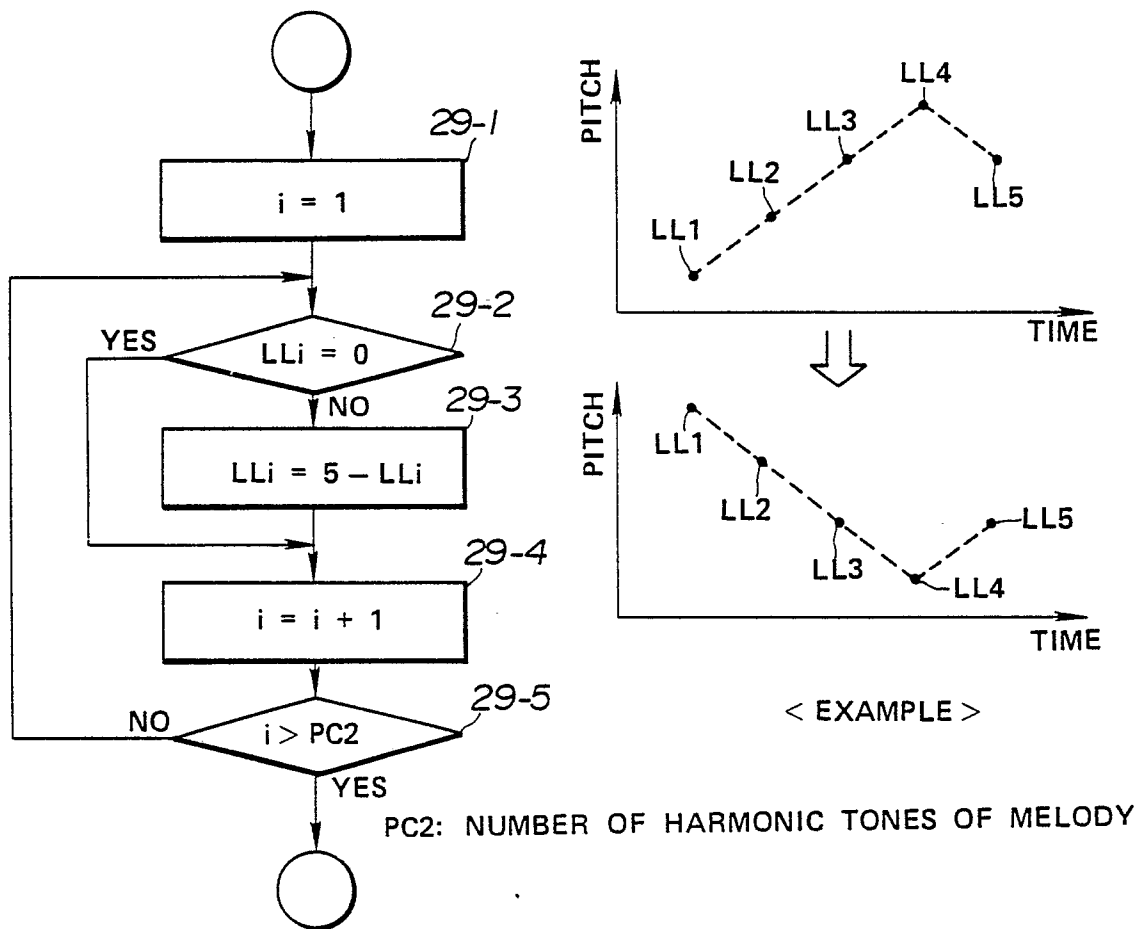
FIG. 29 CORRECT ARPEGGIO PATTERN (DETAILS OF 24-5 IN FIG. 24)
