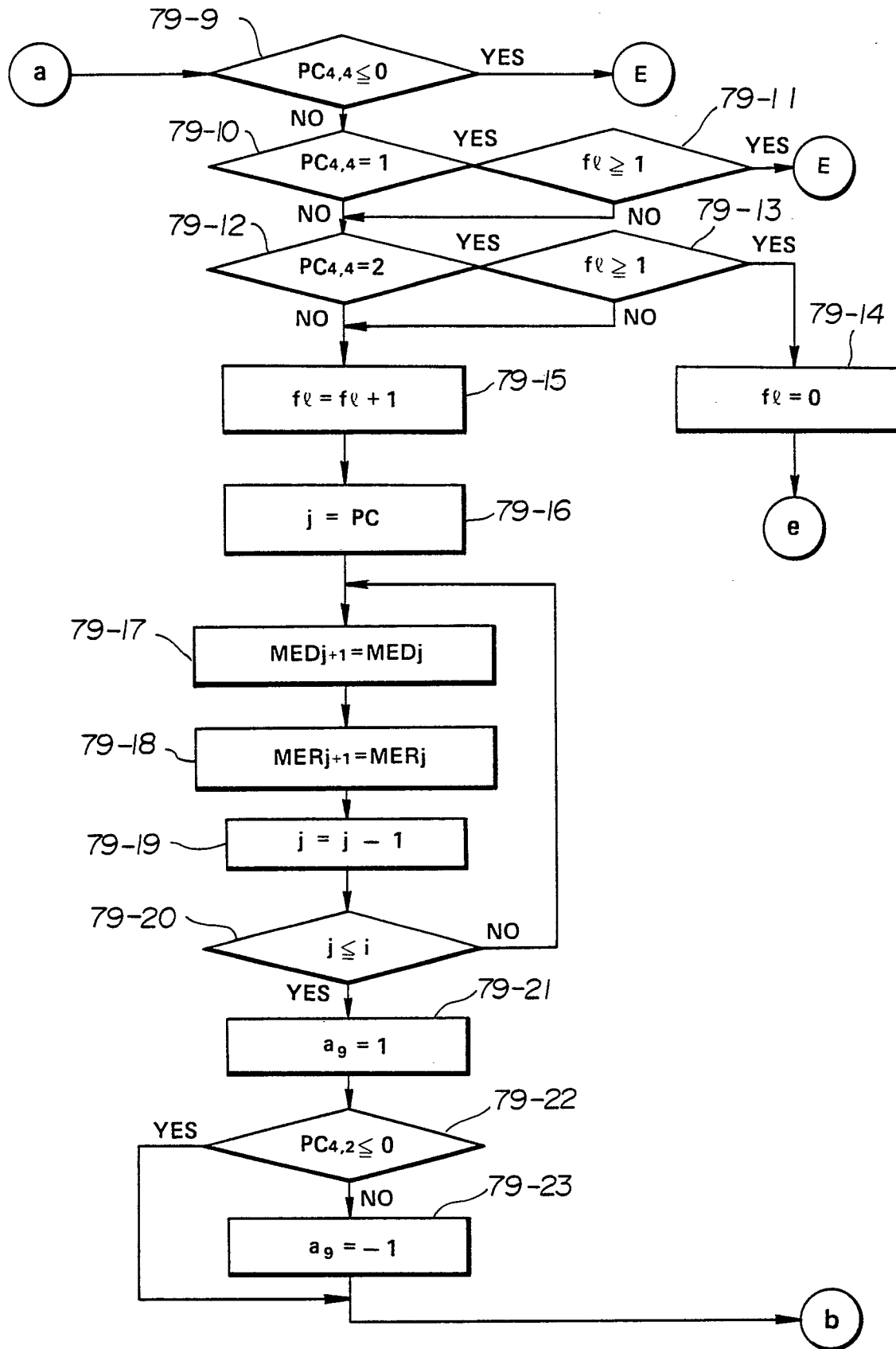
FIG. 79B IMPART NEIGHBOR
