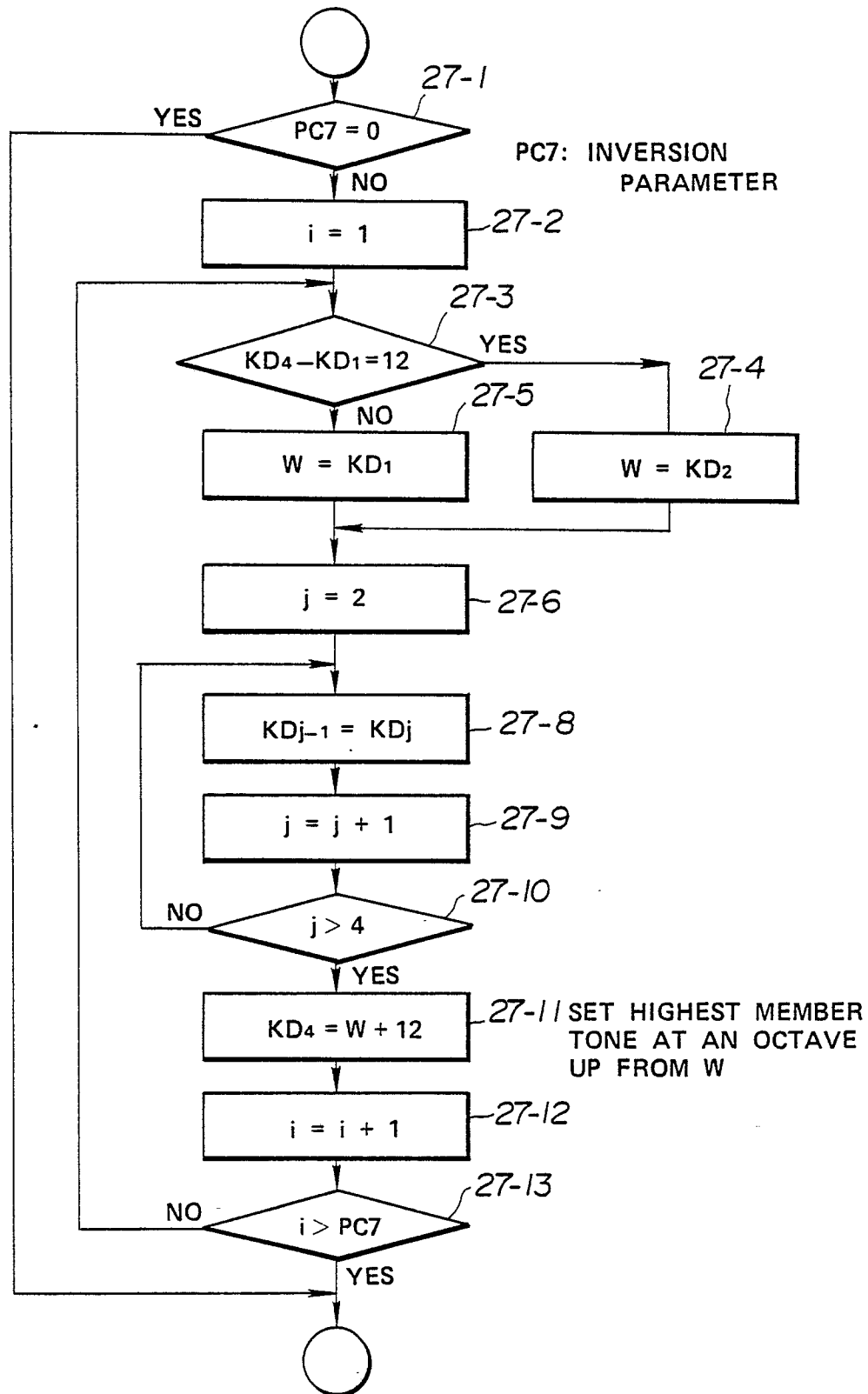
FIG. 27 INVERSION OF CHORD MEMBERS (DETAILS OF 24-2 IN FIG. 24)
