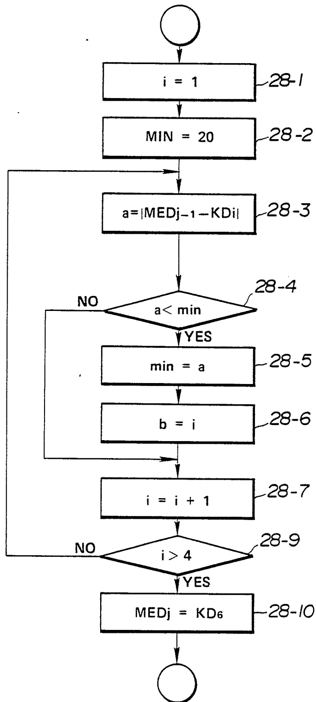
FIG. 28 DETERMINE MED_j FROM PRECEDING TONE (DETAILS OF 24-12 IN FIG. 24)
