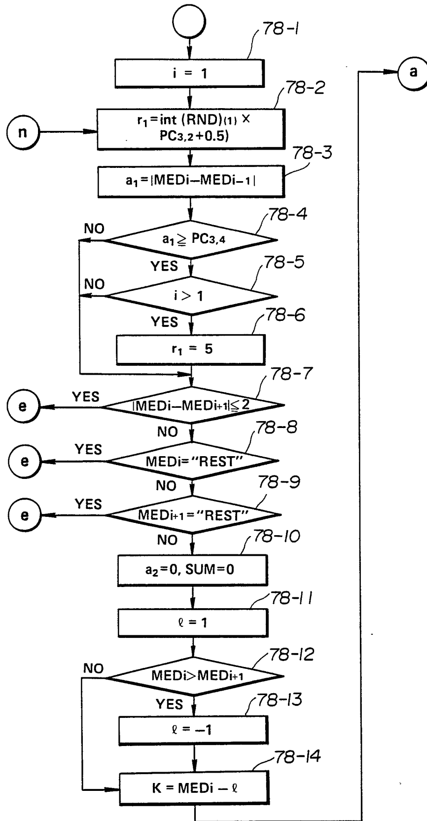
FIG. 78A IMPART PASSING
