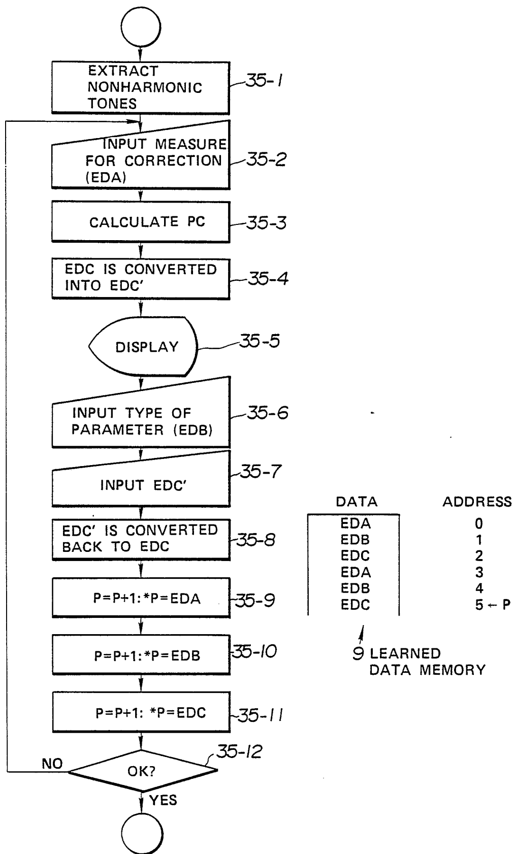
FIG. 35 CORRECT AND LEARN
