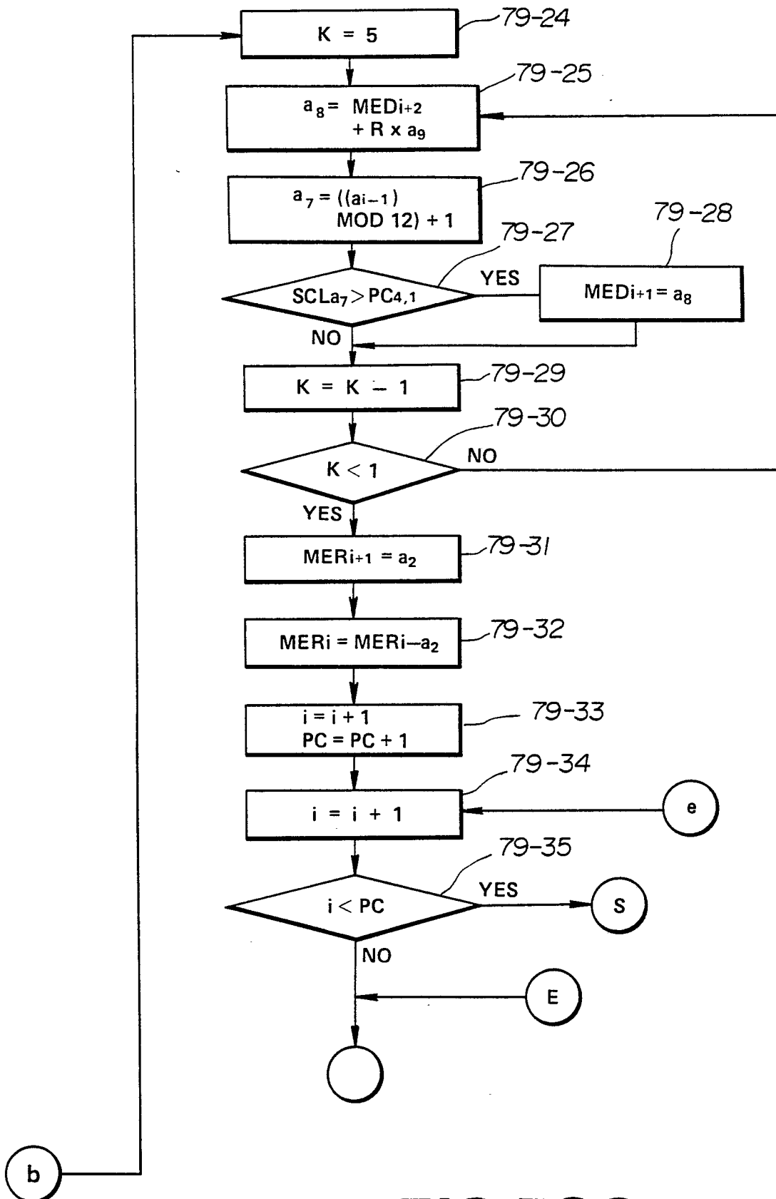
FIG. 79C IMPART NEIGHBOR
