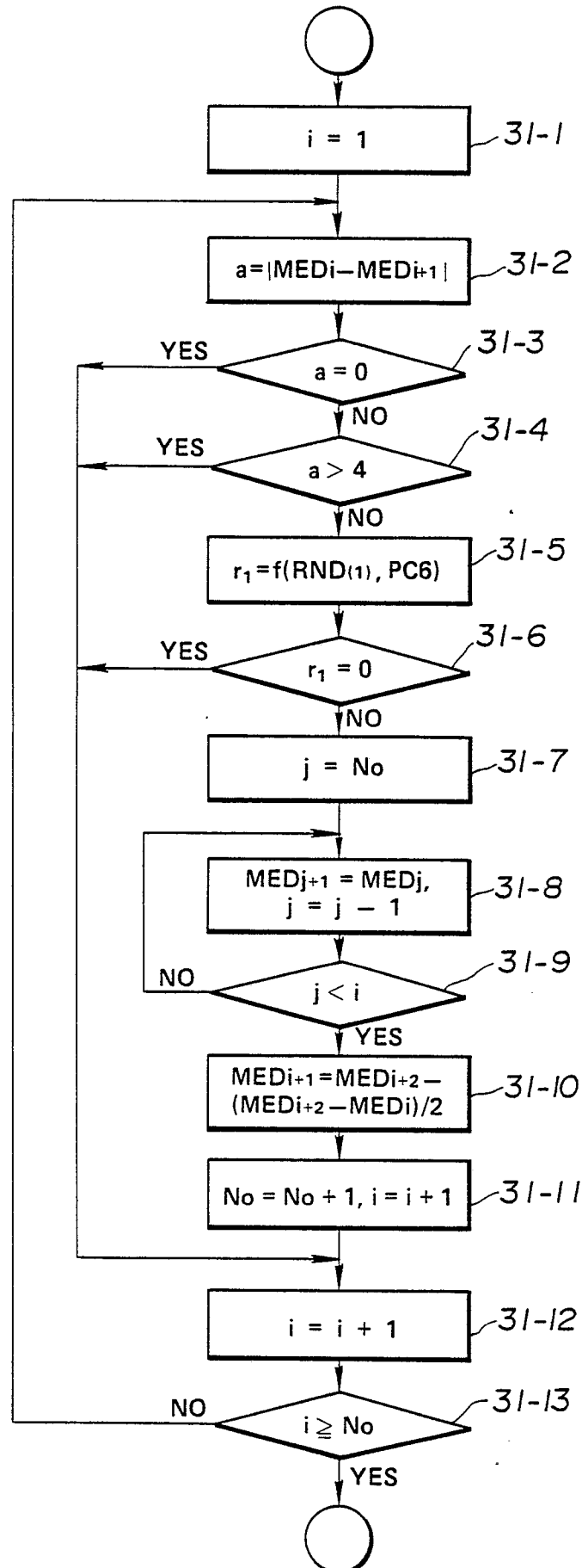
FIG. 31 IMPART PASSING
