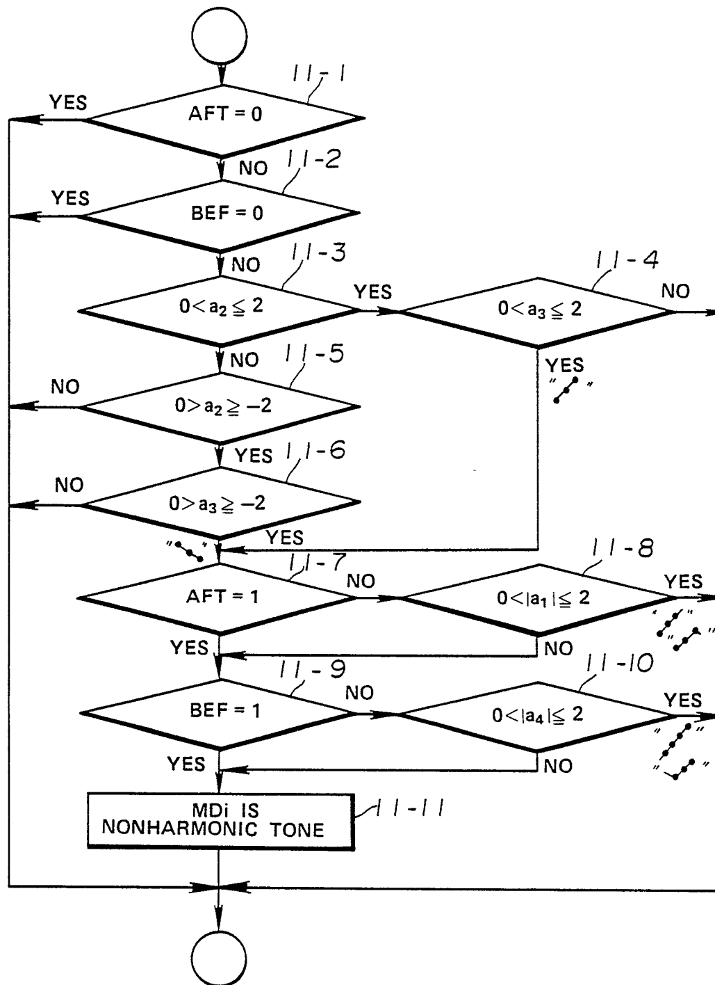
FIG.11 EXTRACT PASSING (DETAILS OF 7-7 IN FIG. 7)
