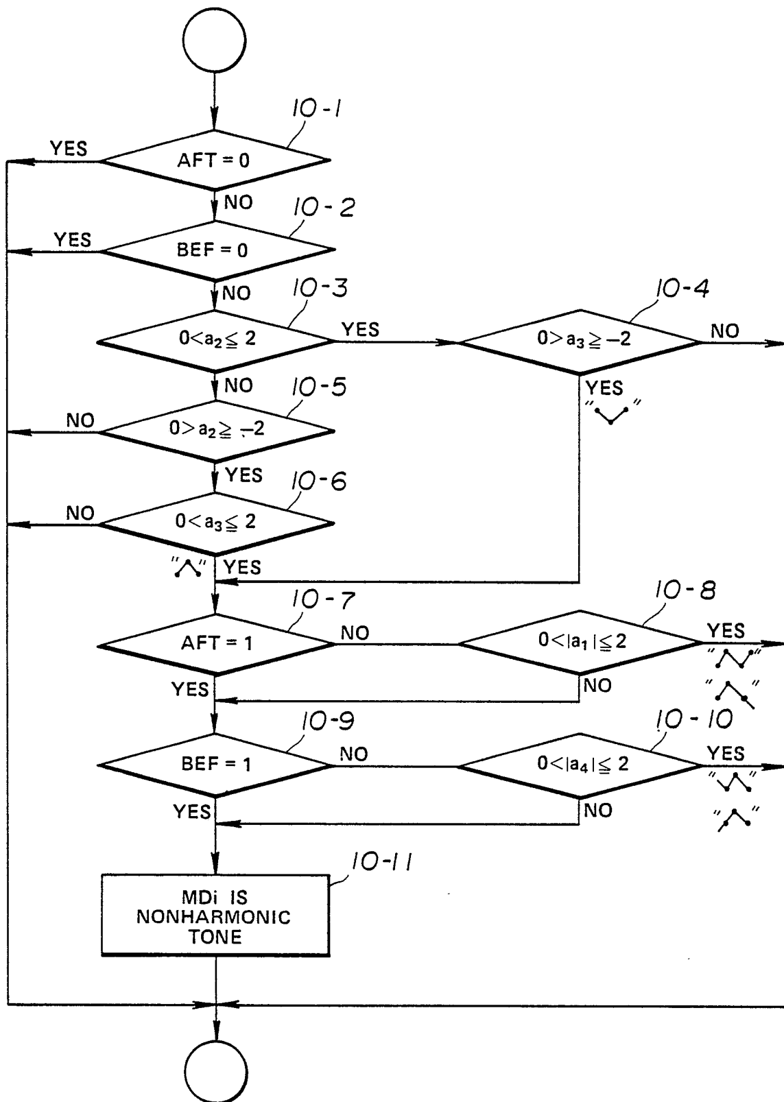
FIG. 10 EXTRACT NEIGHBOR (DETAILS OF 7-6 IN FIG. 7)
