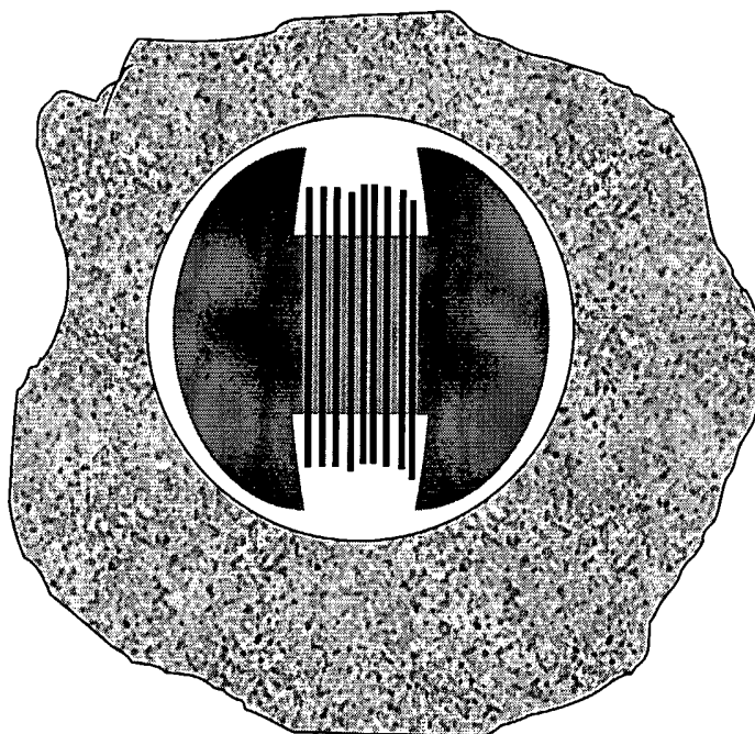
2-pole structure
