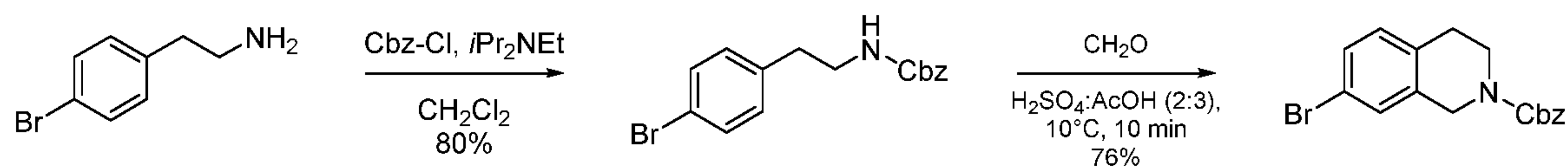
Scheme for Tetrahydroisoquinoline Synthesis
