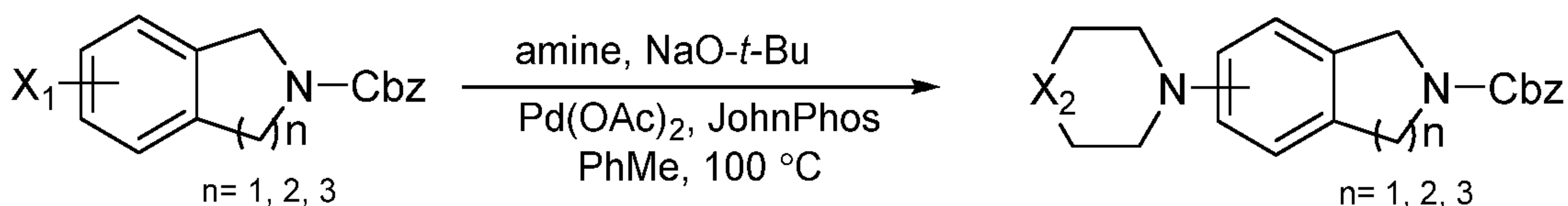
Representative Scheme for Buchwald-Hartwig Amination
