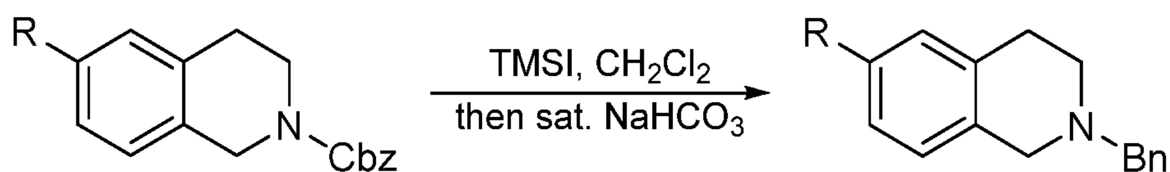
Representative Scheme for TMSI promoted benzylation
