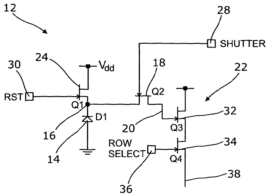
Fig. 4 (Prior Art)
