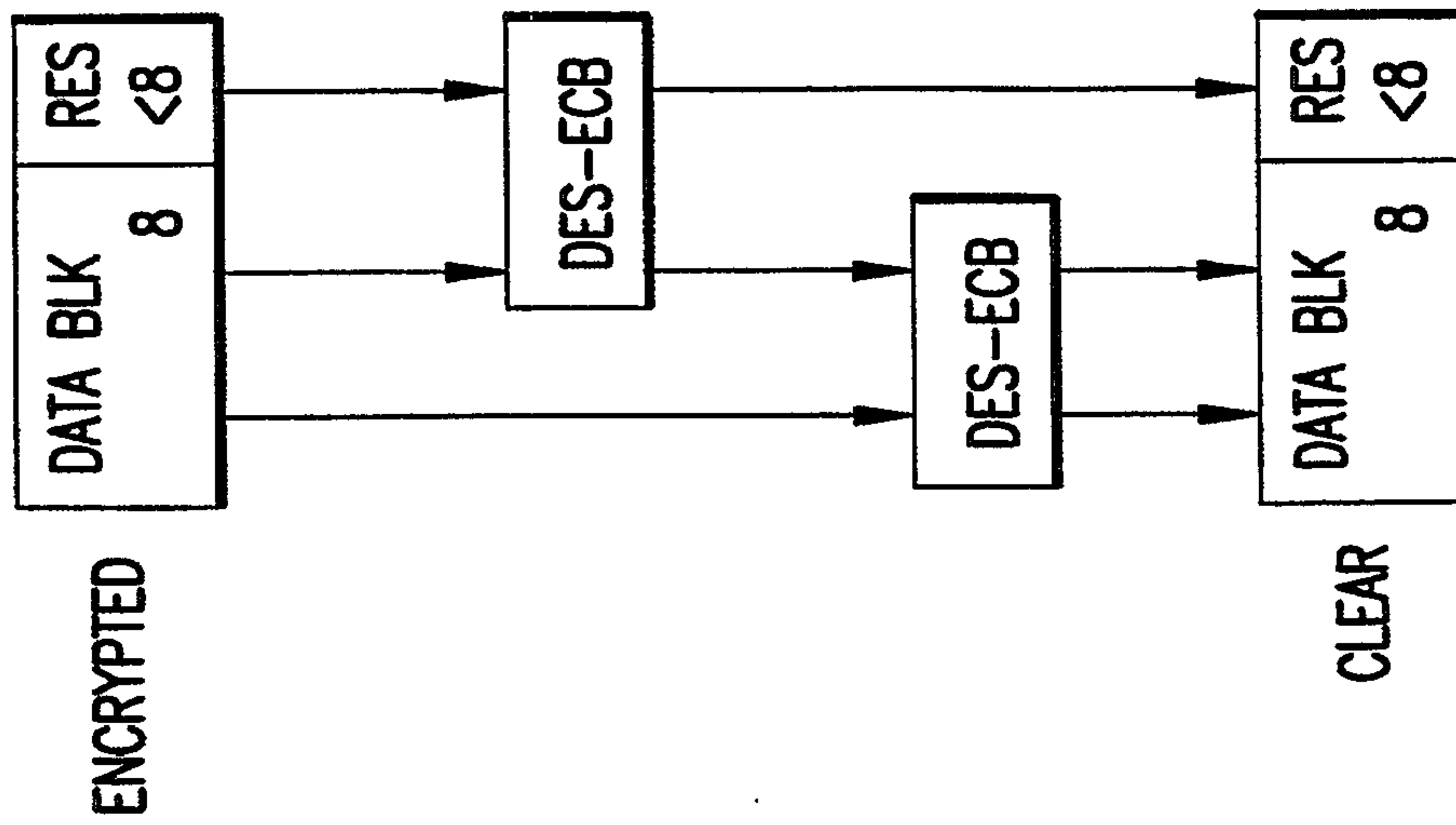
FIG. 6 PRIOR ART
