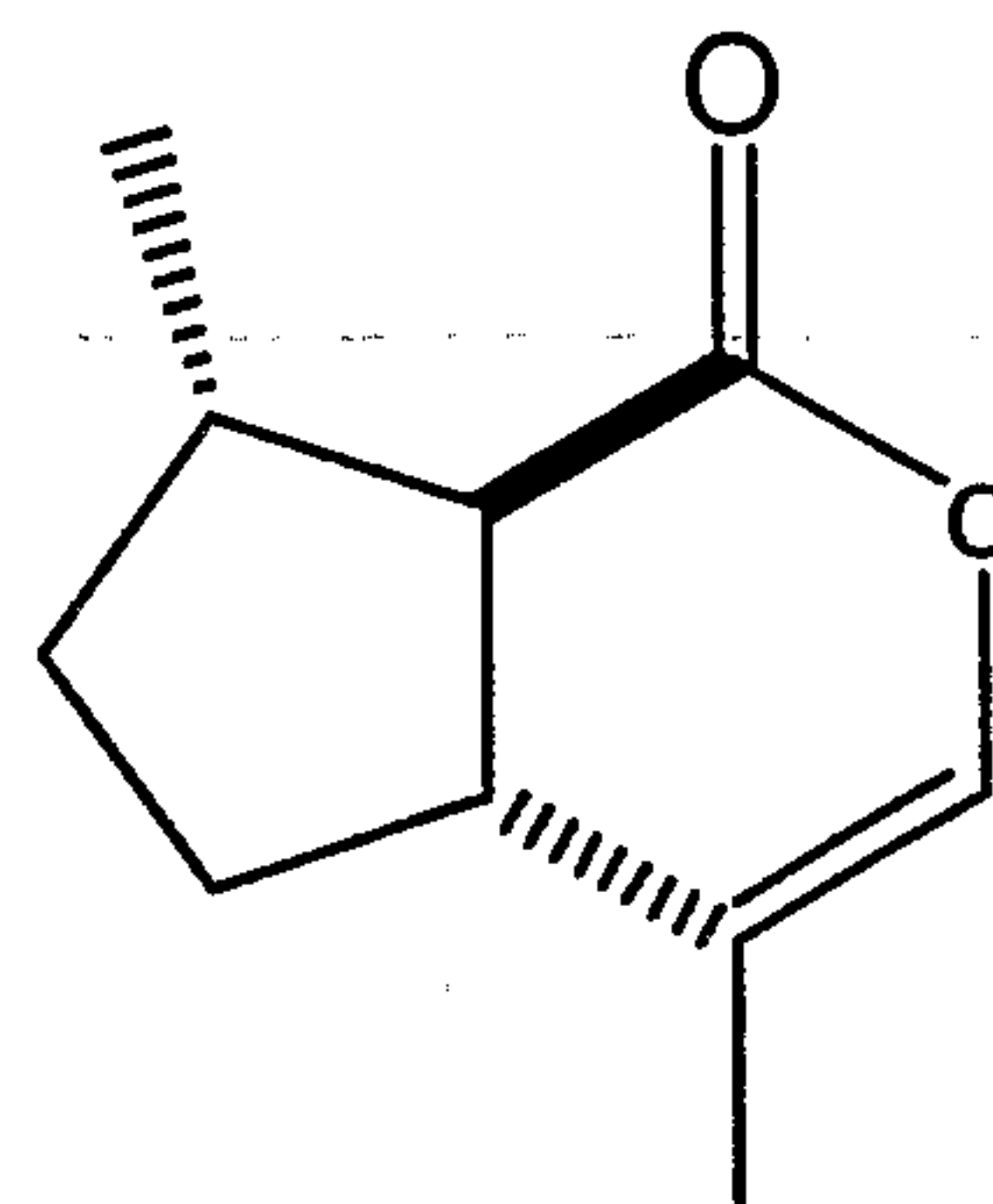
(4aR,7S,7aR) nepetalactone ( trans,trans -nepetalactone)
