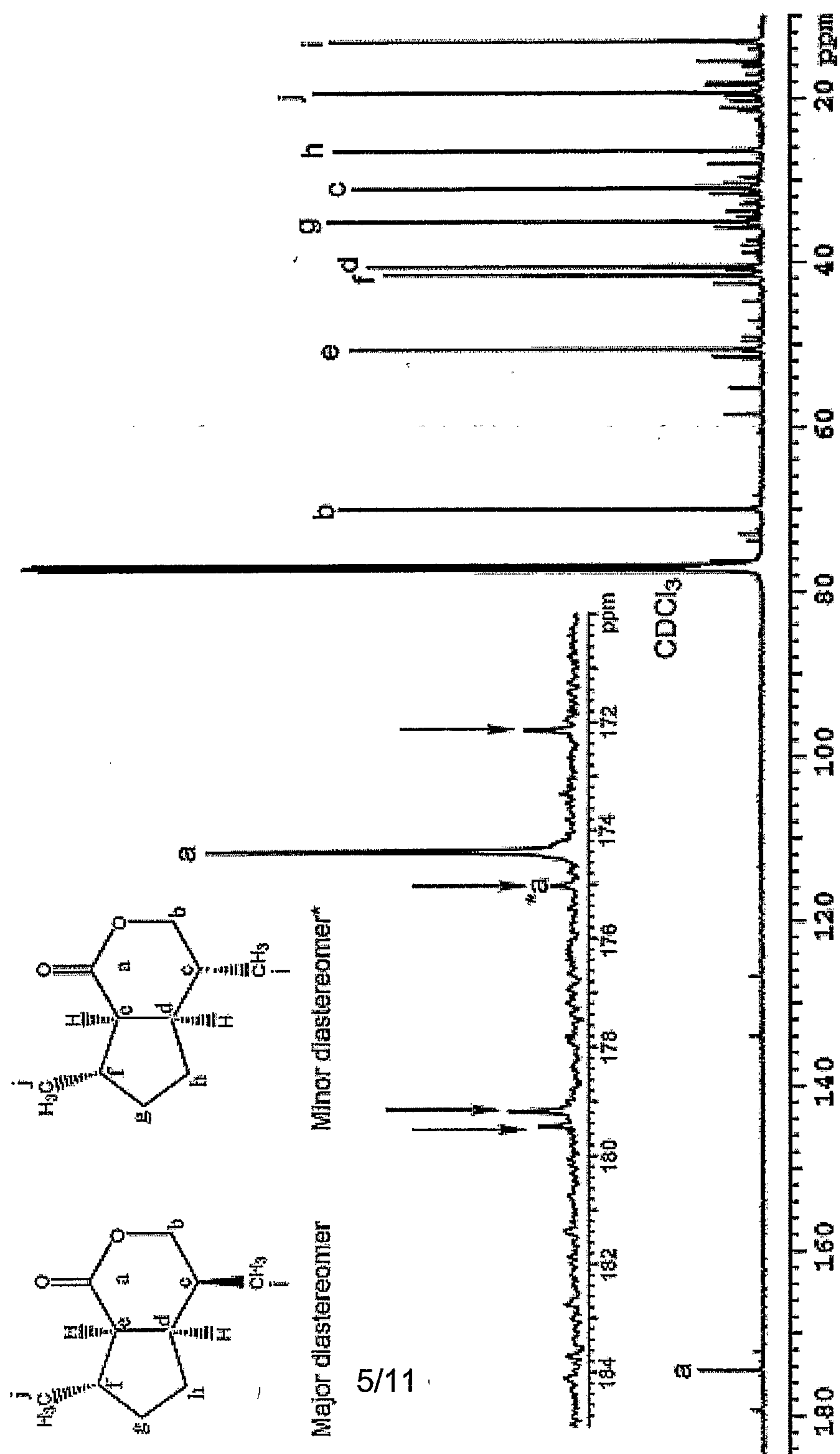
Figure 5 ^{13}\text{C} NMR analysis of dihydronepetalactones in hydrogenated catmint oil.
