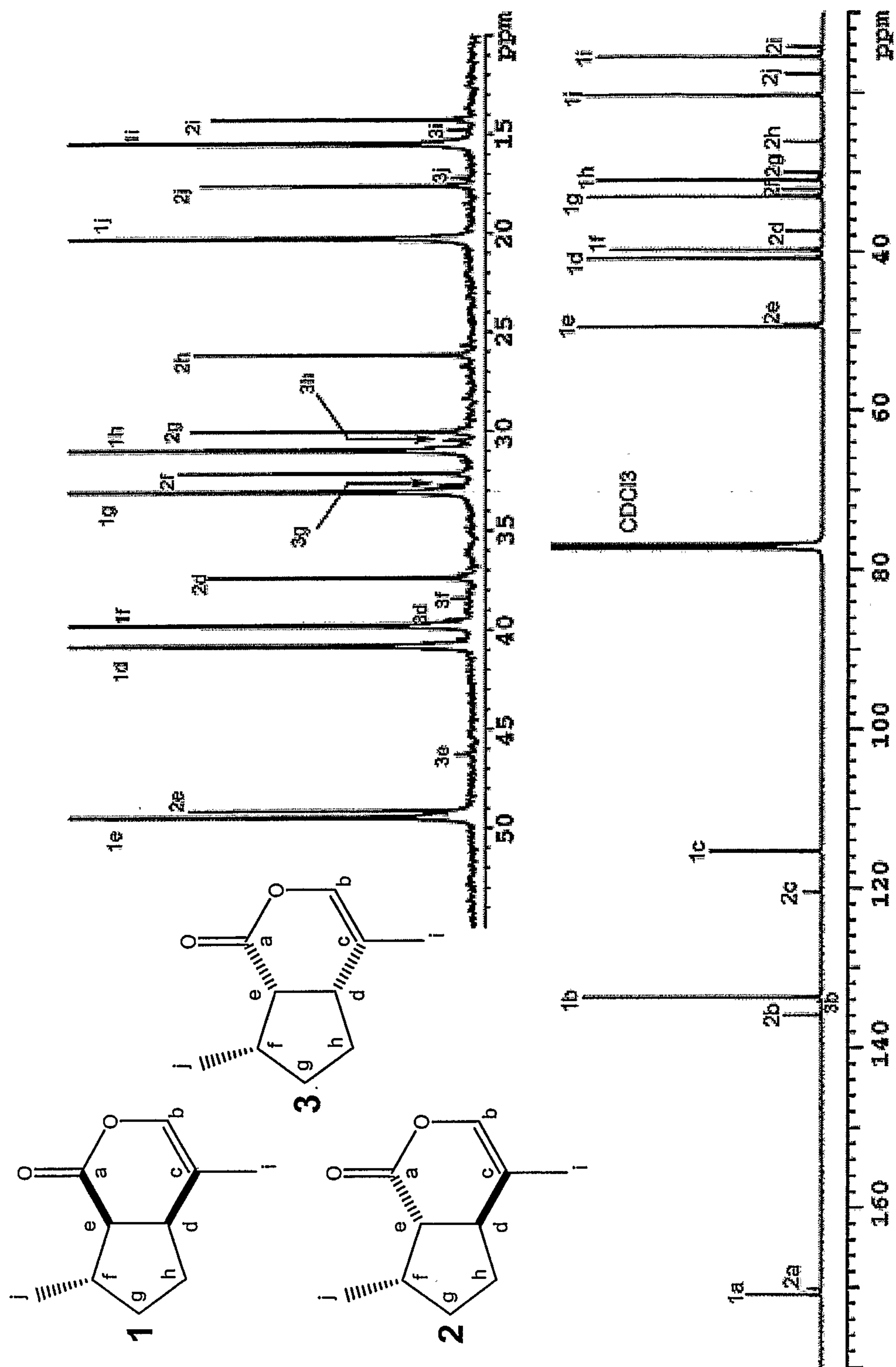
Figure 4 ^{13}\text{C} NMR analysis of nepetalactones in fractionally-distilled catmint oil.
