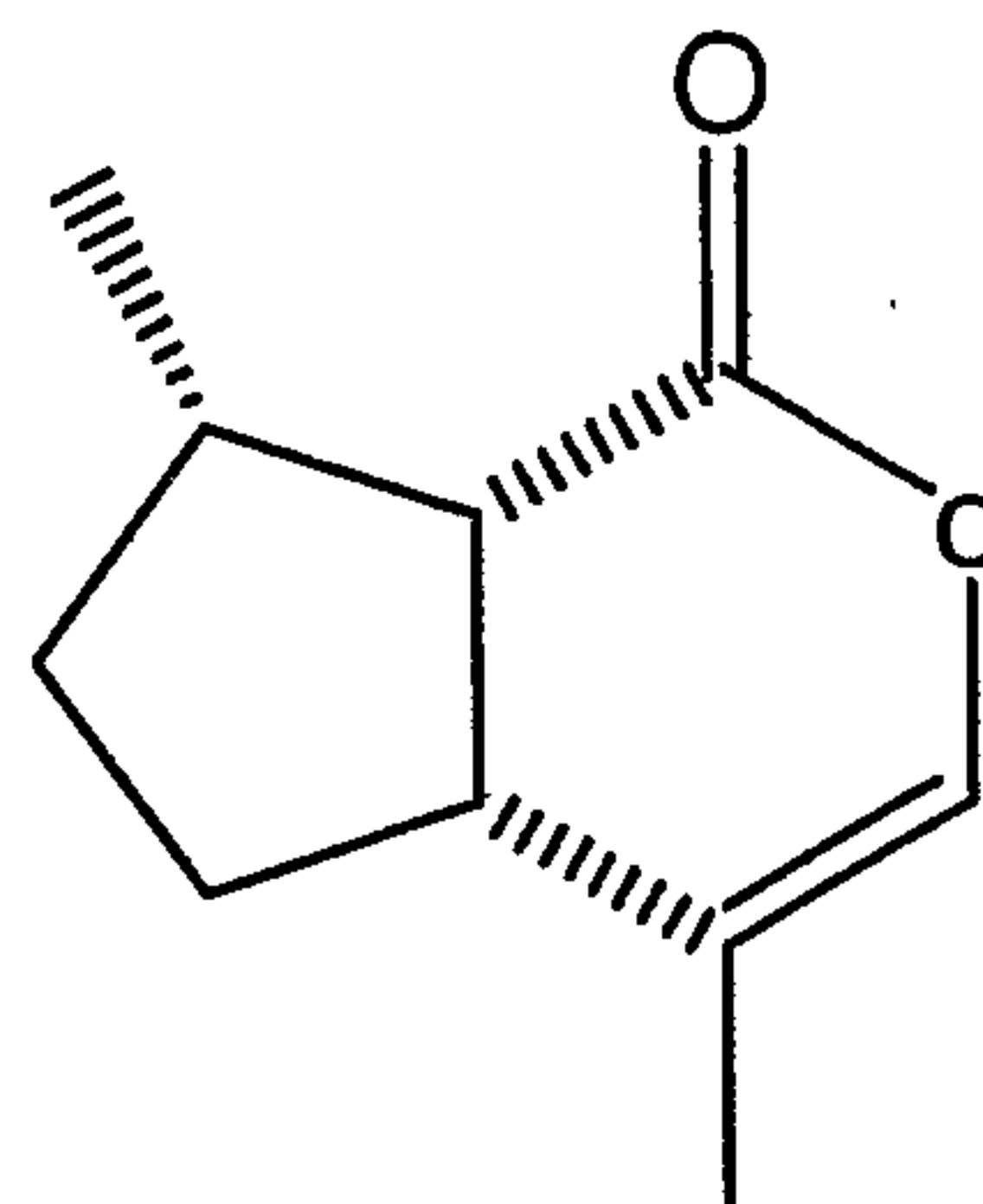
(4aR,7S,7aS) nepetalactone ( cis,cis -nepetalactone)
