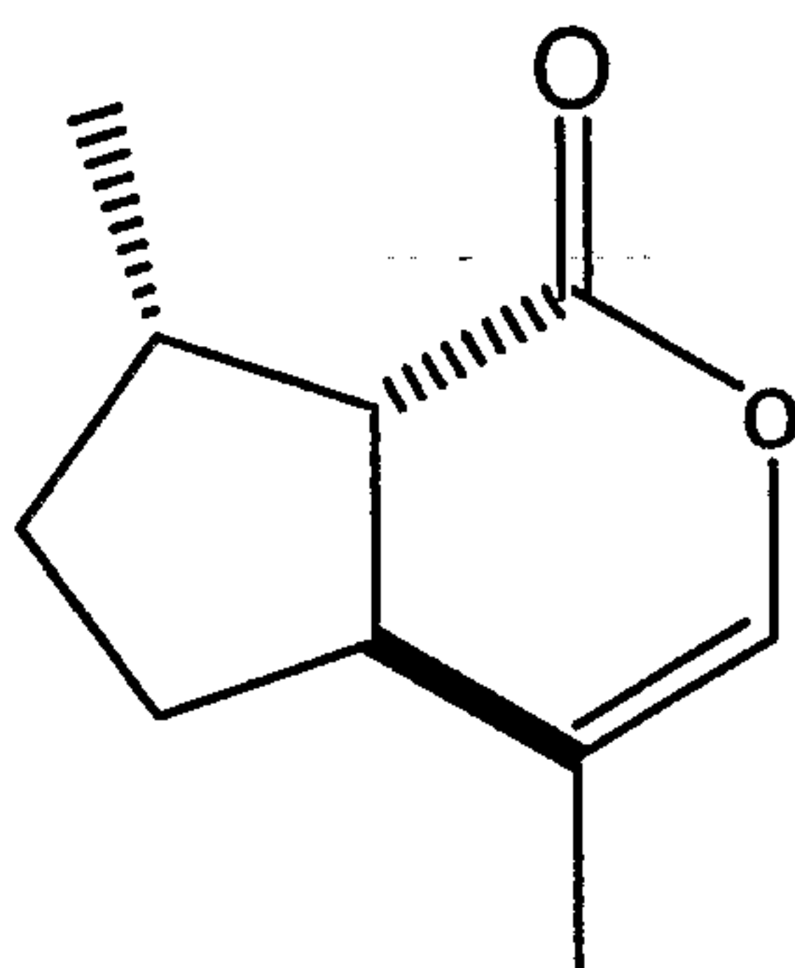
(4aS,7S,7aS) nepetalactone ( trans,cis -nepetalactone)
