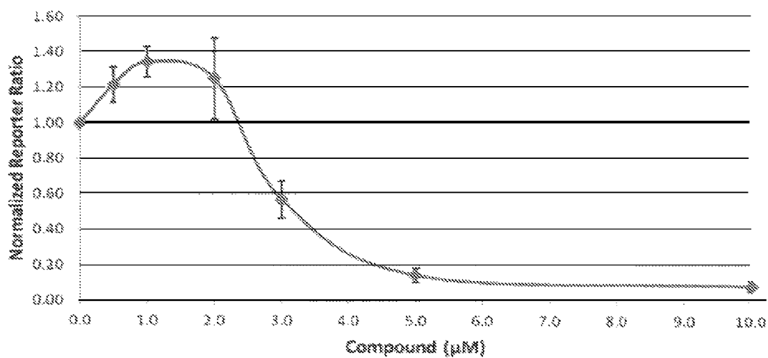
Racemic Mixture of Compounds IV &amp; V
