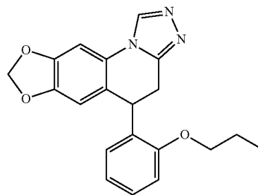
(Structural Formula IX)
