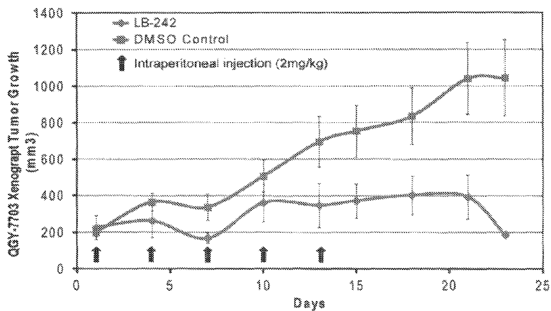
Compound VI – also known as LB-242
