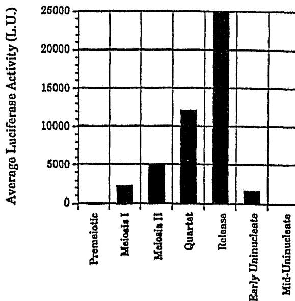
Stage Specificity of MS45 Promoter
