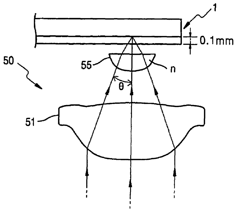
FIG. 2 (PRIOR ART)
