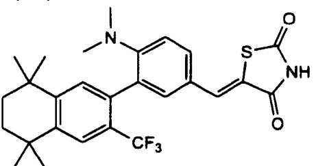
3-(3-Trifluoro-5,5,8,8-tetramethyl-5,6,7,8-tetrahydro-2-naphthyl)-4-dimethylamino benzylidene-2,4-thiazolidinedione
