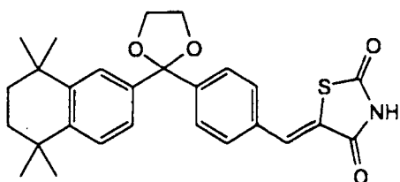
4-[2-(5,5,8,8-Tetramethyl-5,6,7,8-tetrahydro-2-naphthyl)-1,3-dioxolane]benzylidene-2,4-thiazolidinedione
