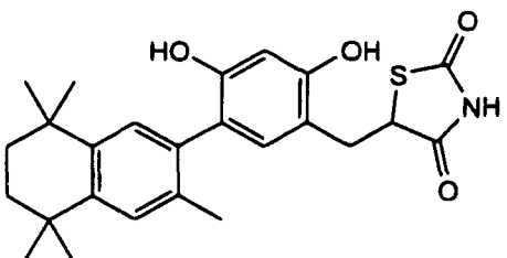
3-(3,5,5,8,8-Pentamethyl-5,6,7,8-tetrahydro-2-naphthyl)-4,6-dihydroxybenzyl-2,4-thiazolidinedione
