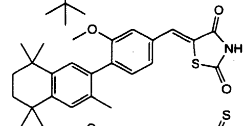
4-(3,5,5,8,8-Pentamethyl-5,6,7,8-tetrahydro-2-naphthyl)-3-methoxybenzylidene-2,4-thiazolidinedione
