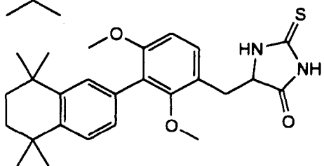
3-(5,5,8,8-Tetramethyl-5,6,7,8-tetrahydro-2-naphthyl)-2,4-dimethoxybenzyl-2-thioxo-4-imidazolidinedione
