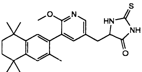
5-[(3,5,5,8,8-Pentamethyl-5,6,7,8-tetrahydro-2-naphthyl)-6-methoxy-3-pyridylmethylene]-2-thioxo-4-imidazolidinedione
