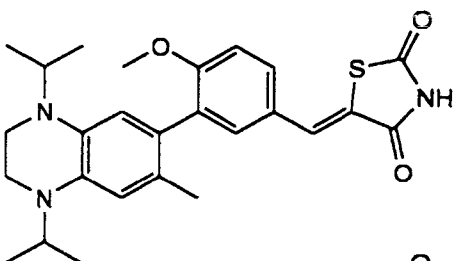
3-(1,4-Diisopropyl-6-methyl-1,2,3,4-tetrahydro-7-quinoxaliny)-4-methoxybenzylidene-2,4-thiazolidinedione
