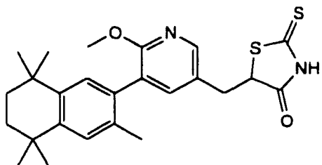
5-(3,5,5,8,8-Pentamethyl-5,6,7,8-tetrahydro-2-naphthyl)-6-methoxy-3-pyridylmethylene-2-thioxo-4-thiazolidinedione
