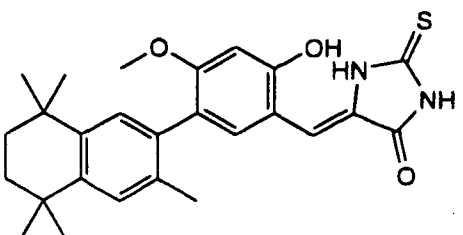
3-(3,5,5,8,8-Pentamethyl-5,6,7,8-tetrahydro-2-naphthyl)-4-methoxy-6-hydroxybenzylidene-2-thioxo-4-imidazolidinedione
