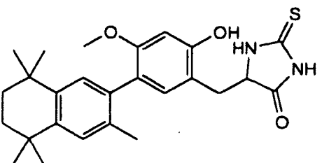
3-(3,5,5,8,8-Pentamethyl-5,6,7,8-tetrahydro-2-naphthyl)-4-methoxy-6-hydroxybenzyl-2-thioxo-4-imidazolidinedione
