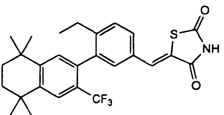
3-(3-Trifluoromethyl-5,5,8,8-tetramethyl-5,6,7,8-tetrahydro-2-naphthyl)-4-ethylbenzylidene-2,4-thiazolidinedione
