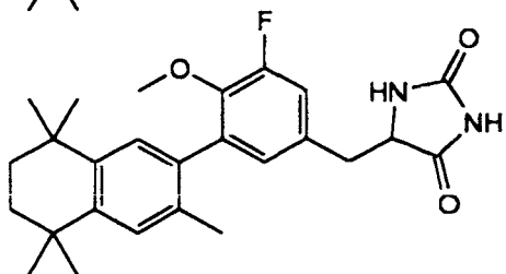
3-(3,5,5,8,8-Pentamethyl-5,6,7,8-tetrahydro-2-naphthyl)-4-methoxy-5-fluorobenzyl-2,4-imidazolidinedione
