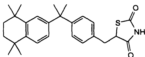
4-[2-(5,5,8,8-Tetramethyl-5,6,7,8-tetrahydro-2-naphthyl)-2-propyl]benzyl-2,4-thiazolidinedione
