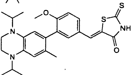
3-(1,4-Diisopropyl-6-methyl-1,2,3,4-tetrahydro-7-quinoxaliny)-4-methoxybenzylidene-2-thioxo-4-thiazolidinedione
