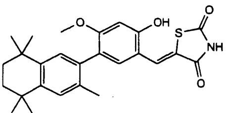
3-(3,5,5,8,8-Pentamethyl-5,6,7,8-tetrahydro-2-naphthyl)-4-methoxy-6-hydroxybenzylidene-2,4-thiazolidinedione
