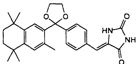
4-[2-(3,5,5,8,8-Tetramethyl-5,6,7,8-tetrahydro-2-naphthyl)-1,3-dioxolane]benzylidene-2,4-imidazolidinedione
