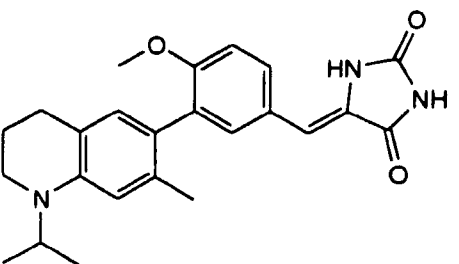
3-(1-Isopropyl-7-methyl-1,2,3,4-tetrahydro-6-quinoliny)-4-methoxybenzylidene-2,4-imidazolidinedione
