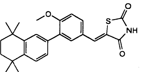
3-(5,5,8,8-Tetramethyl-5,6,7,8-tetrahydro-2-naphthyl)-4-methoxybenzylidene-2,4-thiazolidinedione
