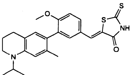
3-(1-Isopropyl-7-methyl-1,2,3,4-tetrahydro-6-quinoliny)-4-methoxybenzylidene-2-thioxo-4-thiazolidinedione
