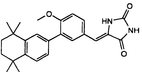
3-(5,5,8,8-Tetramethyl-5,6,7,8-tetrahydro-2-naphthyl)-4-methoxybenzylidene-2,4-imidazolidinedione
