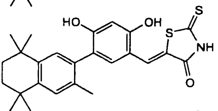
3-(3,5,5,8,8-Pentamethyl-5,6,7,8-tetrahydro-2-naphthyl)-4,6-dihydroxybenzylidene-2-thioxo-4-thiazolidinedione
