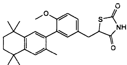
3-[(3,5,5,8,8-Pentamethyl-5,6,7,8-tetrahydro-2-naphthyl)-4-methoxybenzyl]-2,4-thiazolidinedione
