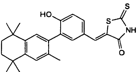
3-(3,5,5,8,8-Pentamethyl-5,6,7,8-tetrahydro-2-naphthyl)-4-hydroxybenzylidene-2-thioxo-4-thiazolidinedione
