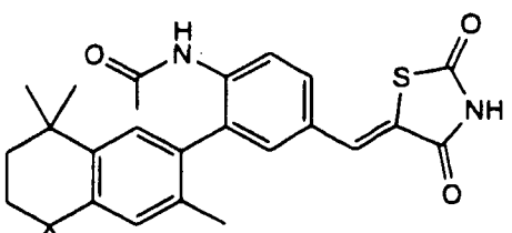
3-(3,5,5,8,8-Pentamethyl-5,6,7,8-tetrahydro-2-naphthyl)-4-acetamidobenzylidene-2,4-thiazolidinedione
