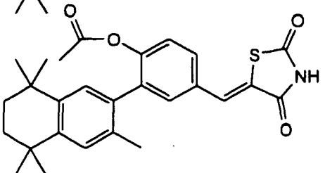
3-(3,5,5,8,8-Pentamethyl-5,6,7,8-tetrahydro-2-naphthyl)-4-acetoxybenzylidene-2,4-thiazolidinedione
