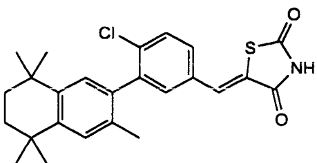
3-(3,5,5,8,8-Pentamethyl-5,6,7,8-tetrahydro-2-naphthyl)-4-chlorobenzylidene-2,4-thiazolidinedione
