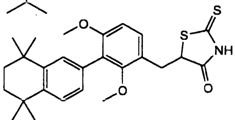
3-(5,5,8,8-Tetramethyl-5,6,7,8-tetrahydro-2-naphthyl)-2,4-dimethoxybenzyl-2-thioxo-4-thiazolidinedione
