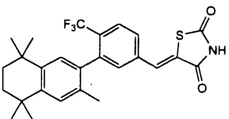
3-(3,5,5,8,8-Pentamethyl-5,6,7,8-tetrahydro-2-naphthyl)-4-trifluoromethylbenzylidene-2,4-thiazolidinedione
