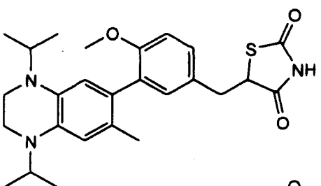
3-(1,4-Diisopropyl-6-methyl-1,2,3,4-tetrahydro-7-quinoxaliny)-4-methoxybenzyl-2,4-thiazolidinedione
