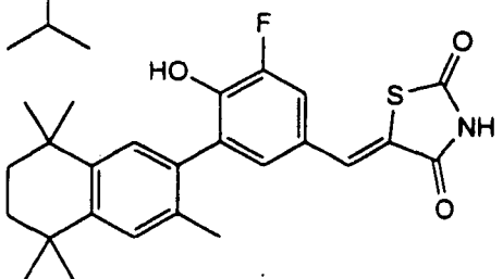
3-(3,5,5,8,8-Pentamethyl-5,6,7,8-tetrahydro-2-naphthyl)-4-hydroxy-5-fluorobenzylidene-2,4-thiazolidinedione
