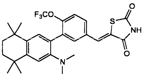
3-(3-Dimethylamino-5,5,8,8-tetramethyl-5,6,7,8-tetrahydro-2-naphthyl)-4-trifluoromethoxybenzylidene-2,4-thiazolidinedione
