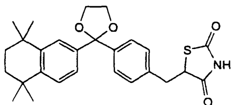
4-[2-(5,5,8,8-Tetramethyl-5,6,7,8-tetrahydro-2-naphthyl)-1,3-dioxolane]benzyl-2,4-thiazolidinedione
