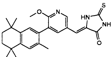
5-(3,5,5,8,8-Pentamethyl-5,6,7,8-tetrahydro-2-naphthyl)-6-methoxy-3-pyridylidene-2-thioxo-4-imidazolidinedione
