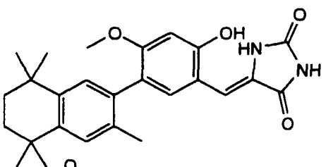
3-(3,5,5,8,8-Pentamethyl-5,6,7,8-tetrahydro-2-naphthyl)-4-methoxy-6-hydroxybenzylidene-2,4-imidazolidinedione
