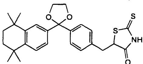
4-[2-(5,5,8,8-Tetramethyl-5,6,7,8-tetrahydro-2-naphthyl)-1,3-dioxolane]benzyl-2-thioxo-4-thiazolidinedione
