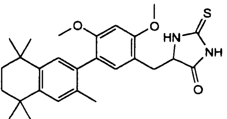
3-(3,5,5,8,8-Pentamethyl-5,6,7,8-tetrahydro-2-naphthyl)-4,6-dimethoxybenzyl-2-thioxo-4-imidazolidinedione,
