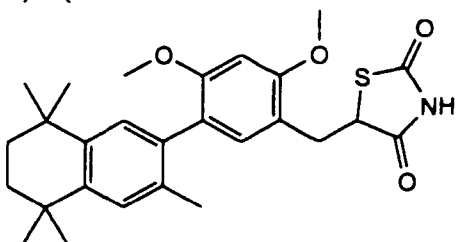
3-(3,5,5,8,8-Pentamethyl-5,6,7,8-tetrahydro-2-naphthyl)-4,6-dimethoxybenzyl-2,4-thiazolidinedione
