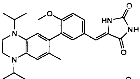
3-(1,4-Diisopropyl-6-methyl-1,2,3,4-tetrahydro-7-quinoxaliny)-4-methoxybenzylidene-2,4-imidazolidinedione
