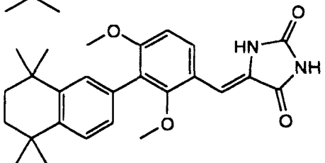
3-(5,5,8,8-Tetramethyl-5,6,7,8-tetrahydro-2-naphthyl)-2,4-dimethoxybenzylidene-2,4-imidazolidinedione
