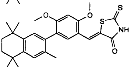
3-(3,5,5,8,8-Pentamethyl-5,6,7,8-tetrahydro-2-naphthyl)-4,6-dimethoxybenzylidene-2-thioxo-4-thiazolidinedione
