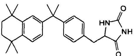
4-[2-(5,5,8,8-Tetramethyl-5,6,7,8-tetrahydro-2-naphthyl)-2-propyl]benzyl-2,4-imidazolidinedione
