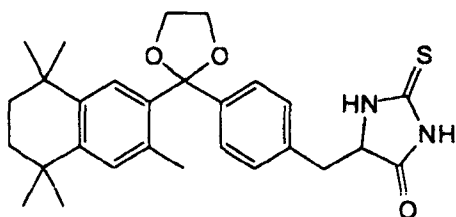
4-[2-(3,5,5,8,8-Pentamethyl-5,6,7,8-tetrahydro-2-naphthyl)-1,3-dioxolane]benzyl-2-thioxo-4-imidazolidinedione
