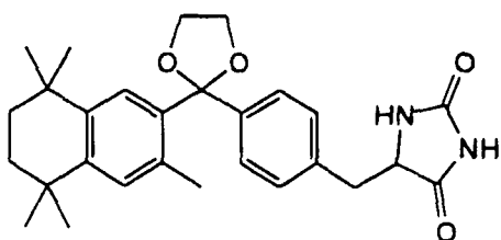
4-[2-(3,5,5,8,8-Pentamethyl-5,6,7,8-tetrahydro-2-naphthyl)-1,3-dioxolane]benzyl-2,4-imidazolidinedione
