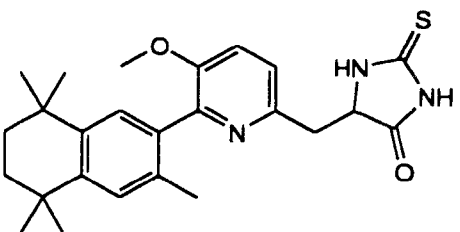
6-[(3,5,5,8,8-Pentamethyl-5,6,7,8-tetrahydro-2-naphthyl)-5-methoxy-2-pyridylmethylene]-2-thioxo-4-imidazolidinedione
