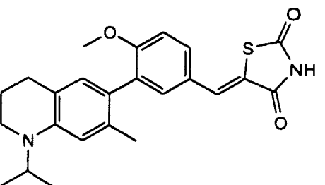
3-(1-Isopropyl-7-methyl-1,2,3,4-tetrahydro-6-quinoliny)-4-methoxybenzylidene-2,4-thiazolidinedione
