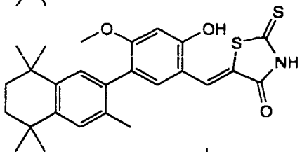
3-(3,5,5,8,8-Pentamethyl-5,6,7,8-tetrahydro-2-naphthyl)-4-methoxy-6-hydroxybenzylidene-2-thioxo-4-thiazolidinedione
