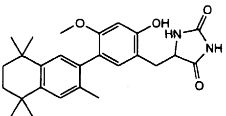
3-(3,5,5,8,8-Pentamethyl-5,6,7,8-tetrahydro-2-naphthyl)-4-methoxy-6-hydroxybenzyl-2,4-imidazolidinedione
