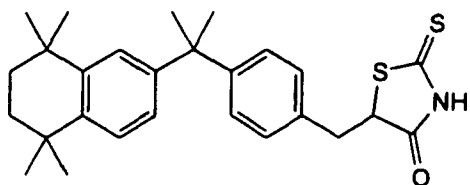
4-[2-(5,5,8,8-Tetramethyl-5,6,7,8-tetrahydro-2-naphthyl)-2-propyl]benzyl-2-thioxo-4-thiazolidinedione
