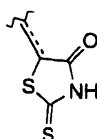
2-thioxo-4-thiazolidinedione
