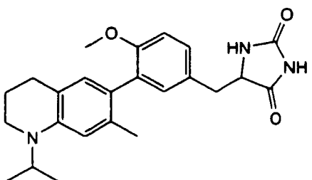
3-(1-Isopropyl-7-methyl-1,2,3,4-tetrahydro-6-quinoliny)-4-methoxybenzyl-2,4-imidazolidinedione
