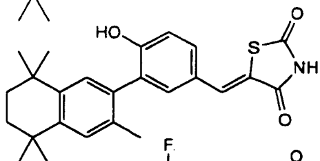
3-(3,5,5,8,8-Pentamethyl-5,6,7,8-tetrahydro-2-naphthyl)-4-hydroxybenzylidene-2,4-thiazolidinedione
