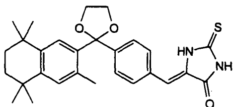
4-[2-(3,5,5,8,8-Tetramethyl-5,6,7,8-tetrahydro-2-naphthyl)-1,3-dioxolane]benzylidene-2-thioxo-4-imidazolidinedione
