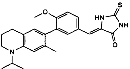
3-(1-Isopropyl-7-methyl-1,2,3,4-tetrahydro-6-quinoliny)-4-methoxybenzylidene-2-thioxo-4-imidazolidinedione
