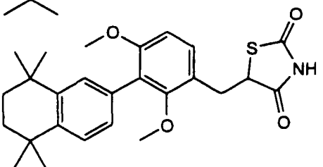
3-(5,5,8,8-Tetramethyl-5,6,7,8-tetrahydro-2-naphthyl)-2,4-dimethoxybenzyl-2,4-thiazolidinedione
