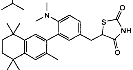
3-(3,5,5,8,8-Pentamethyl-5,6,7,8-tetrahydro-2-naphthyl)-4-dimethylaminobenzyl-2,4-thiazolidinedione
