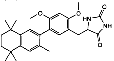
3-(3,5,5,8,8-Pentamethyl-5,6,7,8-tetrahydro-2-naphthyl)-4,6-dimethoxybenzyl-2,4-imidazolidinedione
