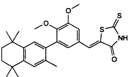
3-(3,5,5,8,8-Pentamethyl-5,6,7,8-tetrahydro-2-naphthyl)-4,5-dimethoxybenzylidene-2-thioxo-4-thiazolidinedione
