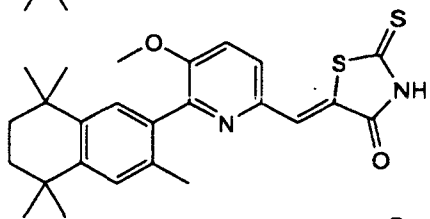
6-(3,5,5,8,8-Pentamethyl-5,6,7,8-tetrahydro-2-naphthyl)-5-methoxy-2-pyridylidene-2-thioxo-4-thiazolidinedione
