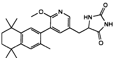
5-[(3,5,5,8,8-Pentamethyl-5,6,7,8-tetrahydro-2-naphthyl)-6-methoxy-3-pyridylmethylene]-2,4-imidazolidinedione
