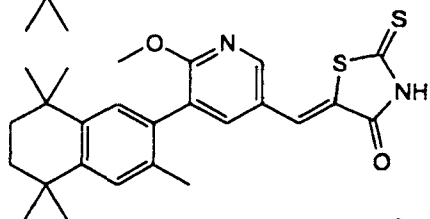
5-(3,5,5,8,8-Pentamethyl-5,6,7,8-tetrahydro-2-naphthyl)-6-methoxy-3-pyridylidene-2-thioxo-4-thiazolidinedione
