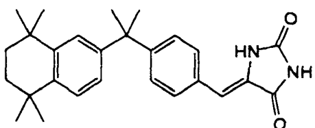
4-[2-(5,5,8,8-Tetramethyl-5,6,7,8-tetrahydro-2-naphthyl)-2-propyl]benzylidene-2,4-imidazolidinedione
