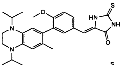
3-(1,4-Diisopropyl-6-methyl-1,2,3,4-tetrahydro-7-quinoxaliny)-4-methoxybenzylidene-2-thioxo-4-imidazolidinedione
