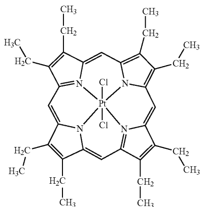
PtCl 2 OEP
