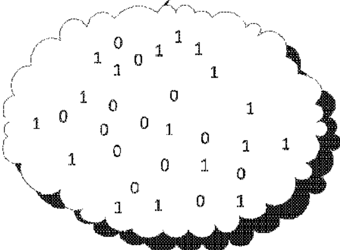
Ciphertext
