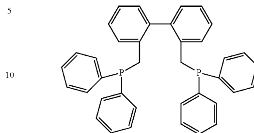
FIG. 2. Comparative Ligand B; BISBI.
