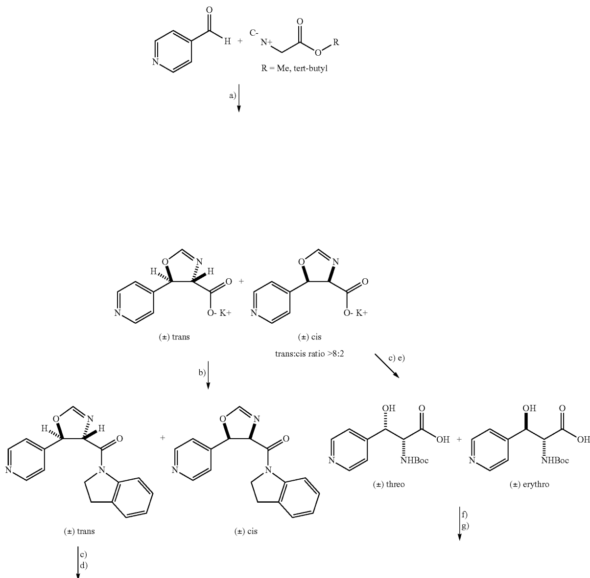
Reaction Scheme 2
