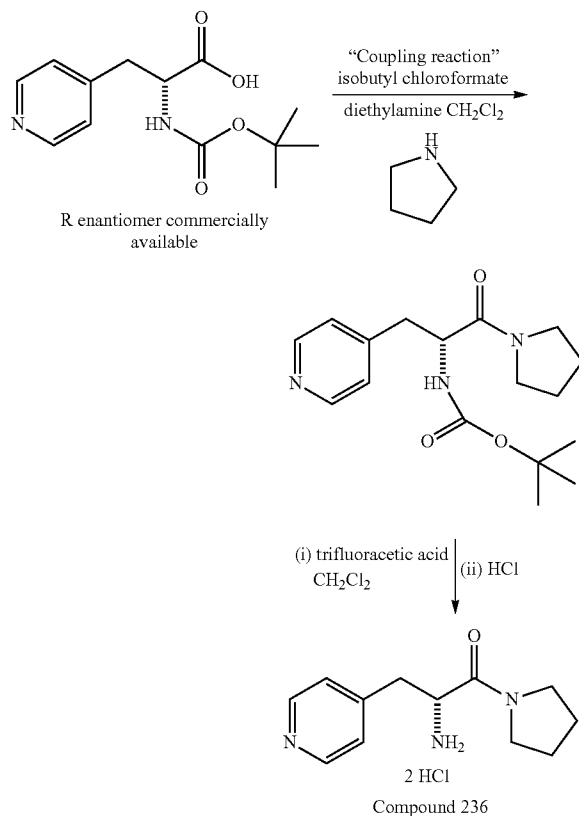
Synthetic Scheme 3
