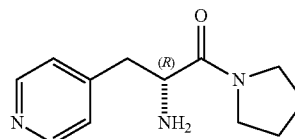
2 HCl
