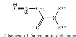
R*—CHO "aldehyde"
