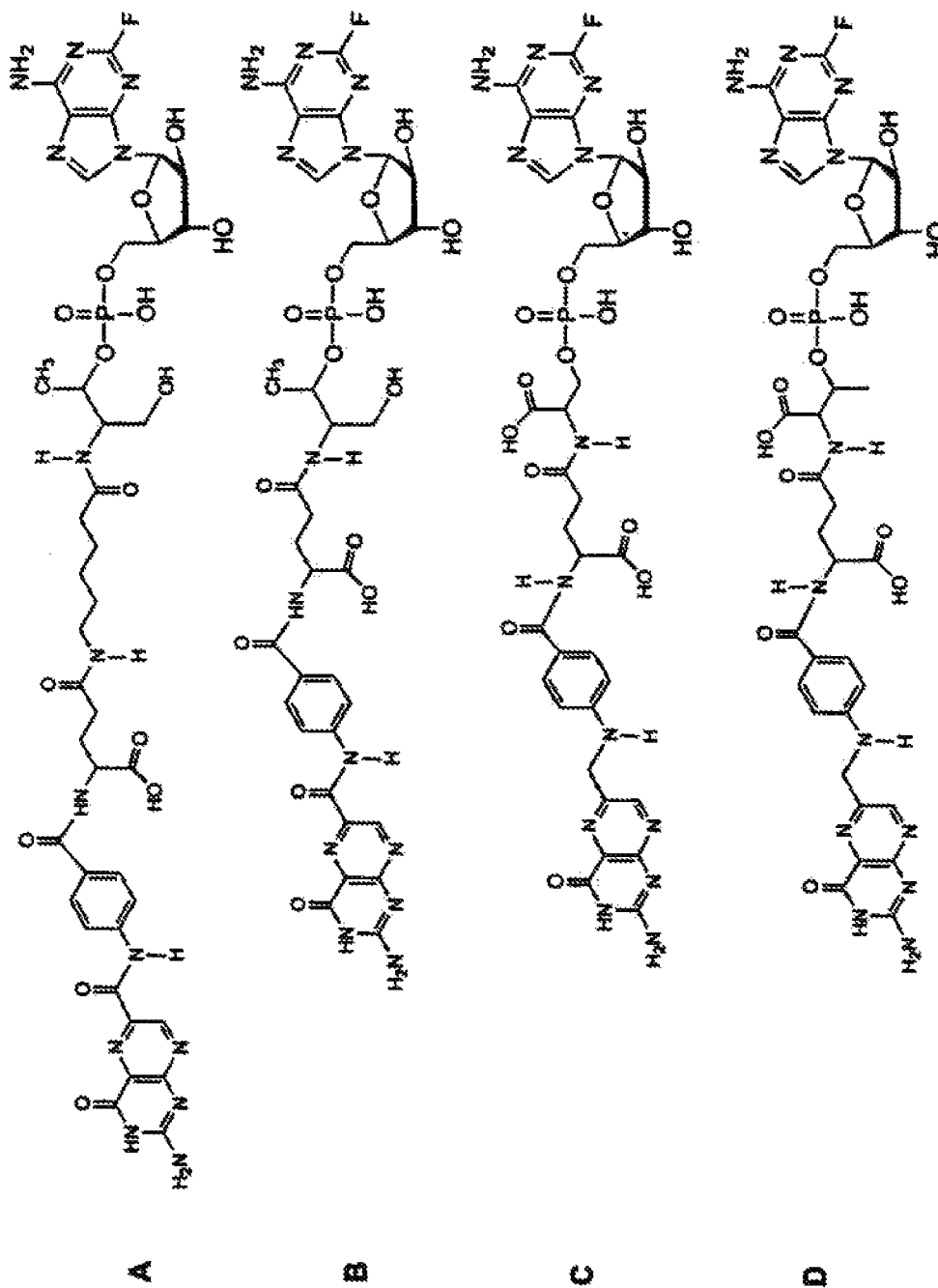
Figure 6: Fludarabine-Folate conjugates
