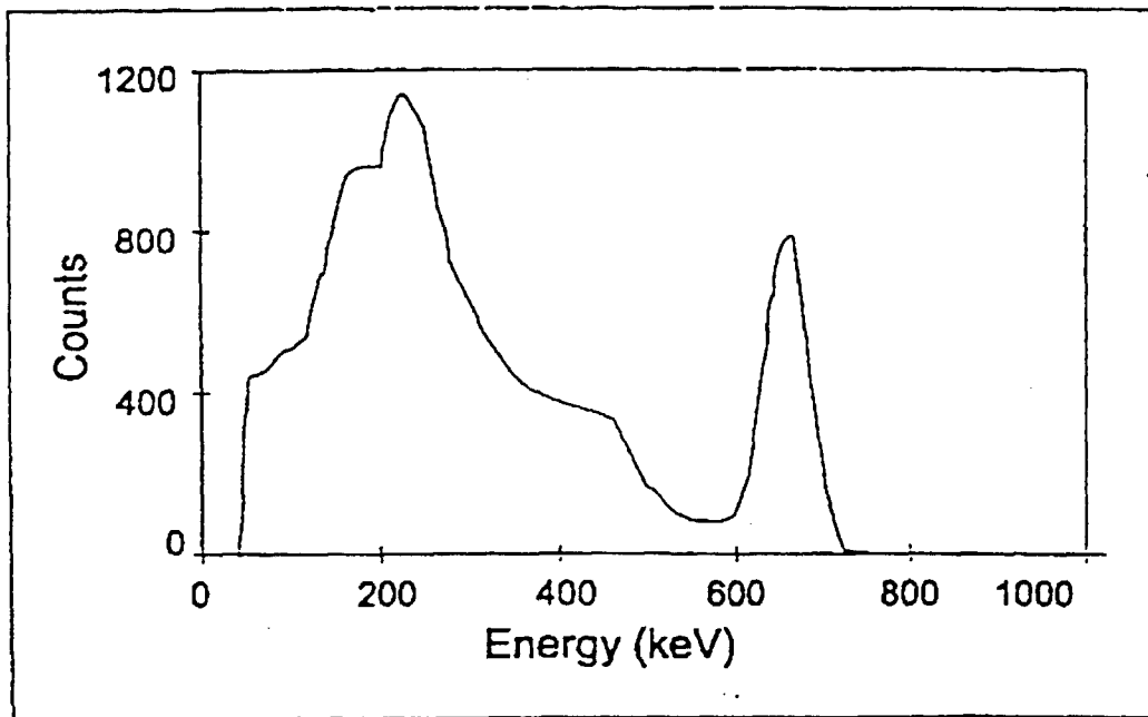
Figure 1. Spectrum from a stabilization source placed on the far detector of a wireline density tool.
