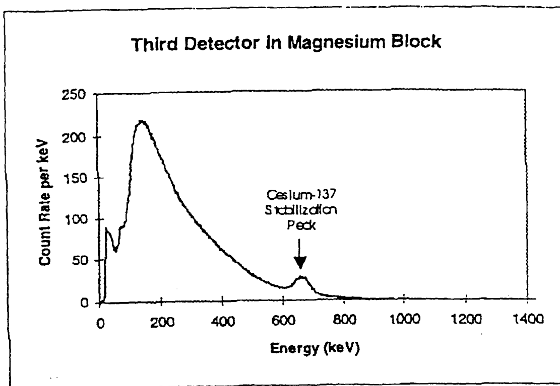
Figure 4 Combined Logging and Stabilization spectrum for the third detector of a cased-hole density tool placed in a magnesium block.
