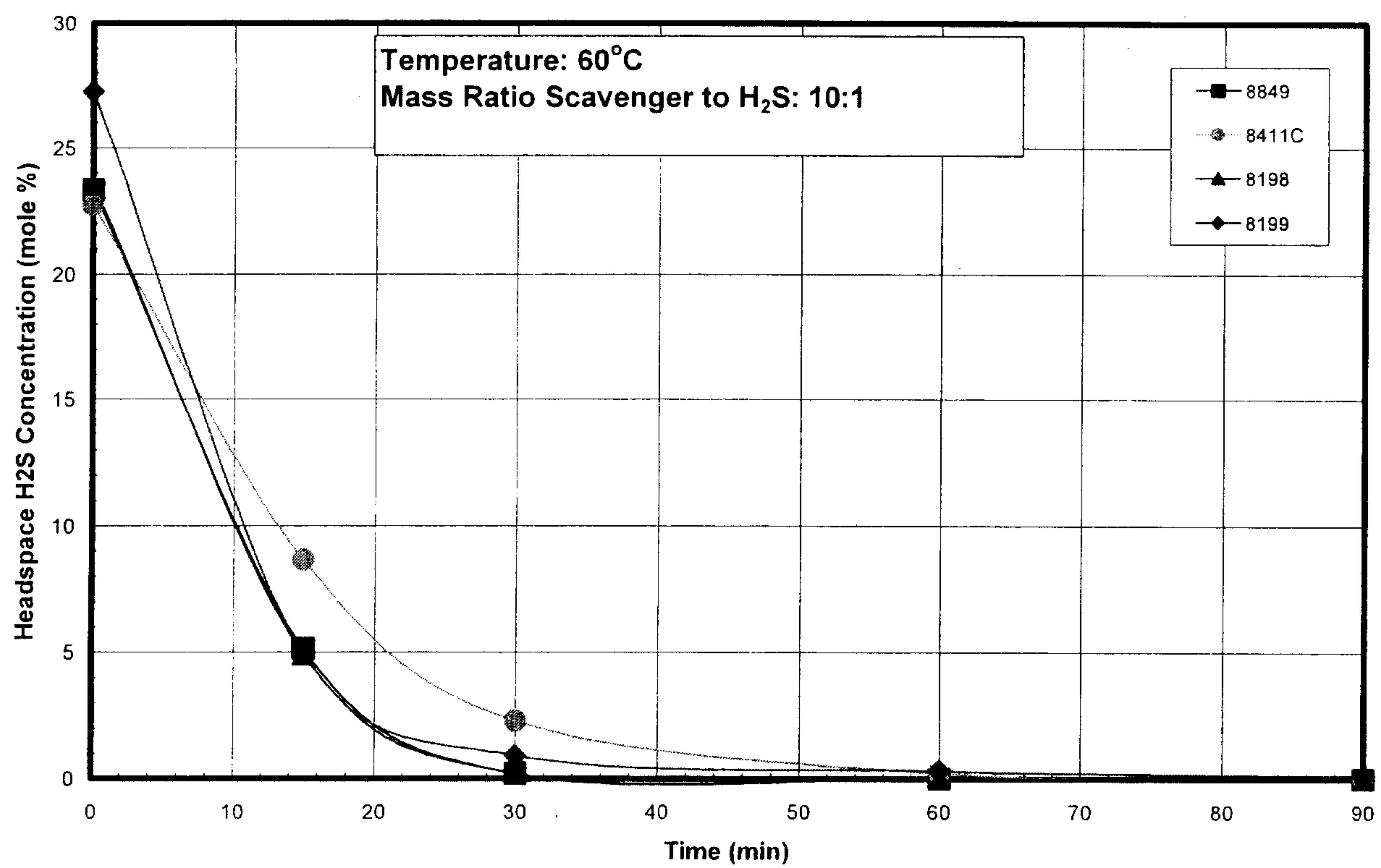
Fig. 6 : Comparison of Scavenger Efficiency
