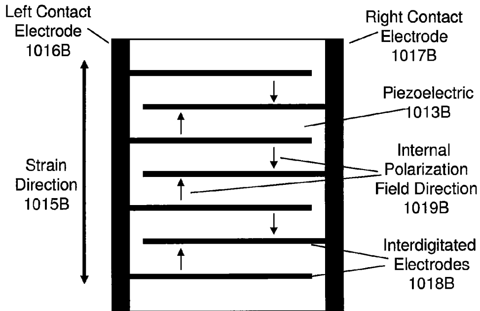
Interdigitated Piezoelectric 1030B
