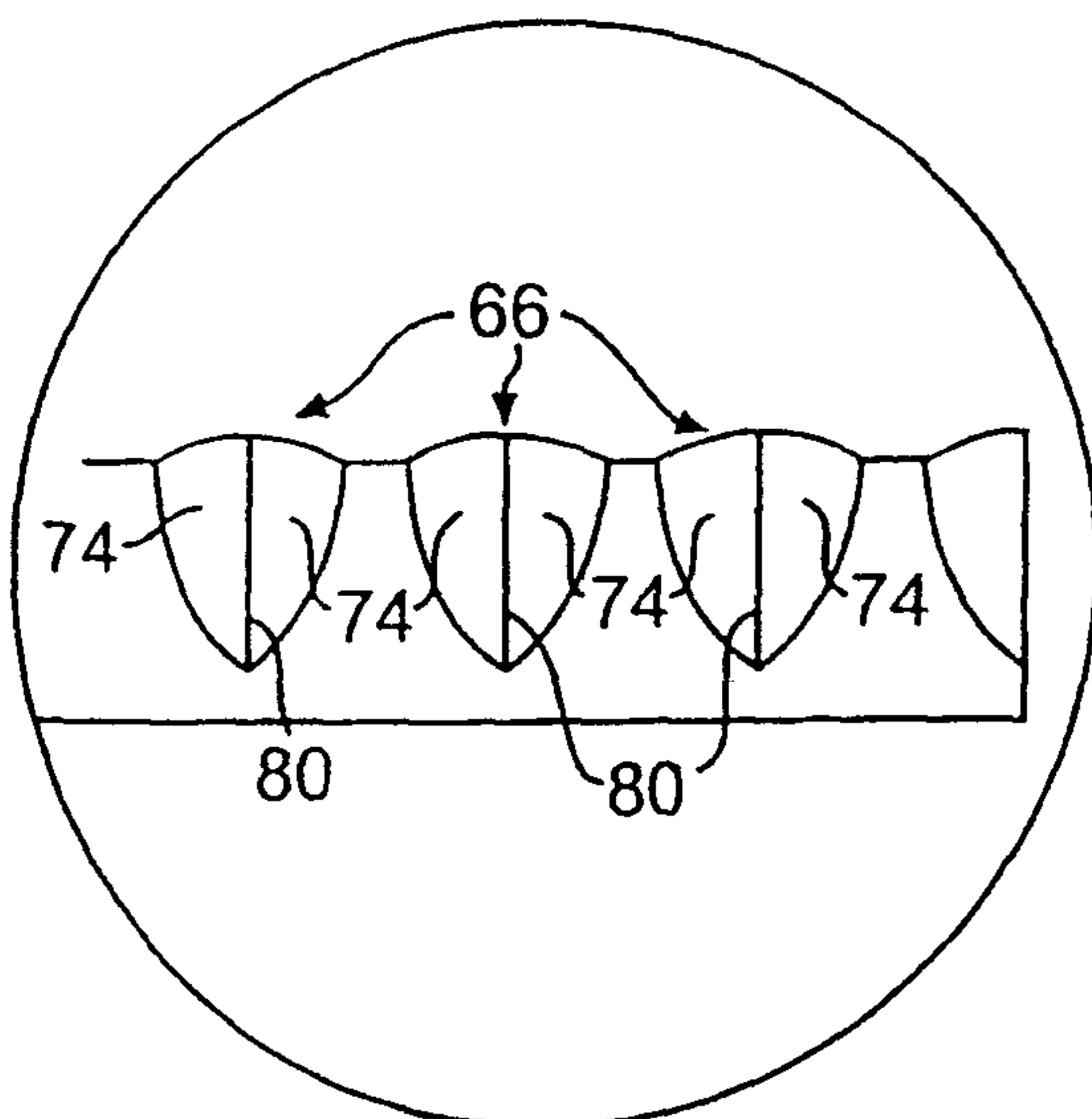
FIG. 8F (PRIOR ART)
