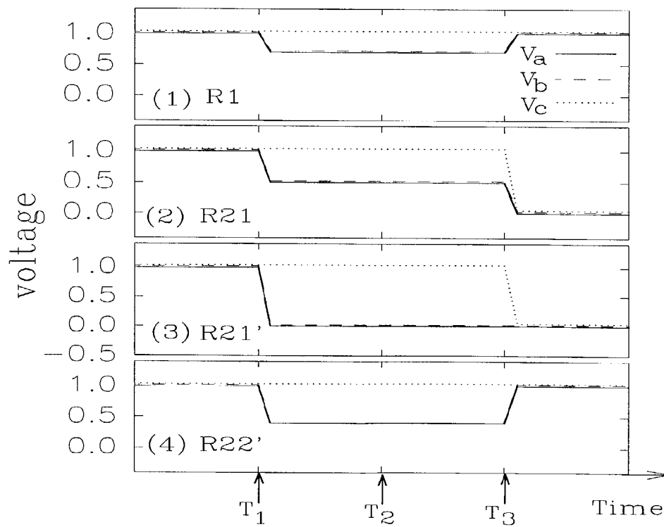
Figure 4b (Fault phase 'a'-b' on Line L21)
