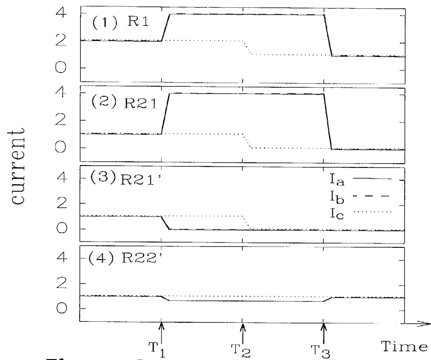
Figure 4a (Fault phase 'a'-b' on Line L21)
