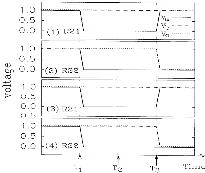
Figure 5b (Fault phase 'a'-e' on Line L22 near busbar)
