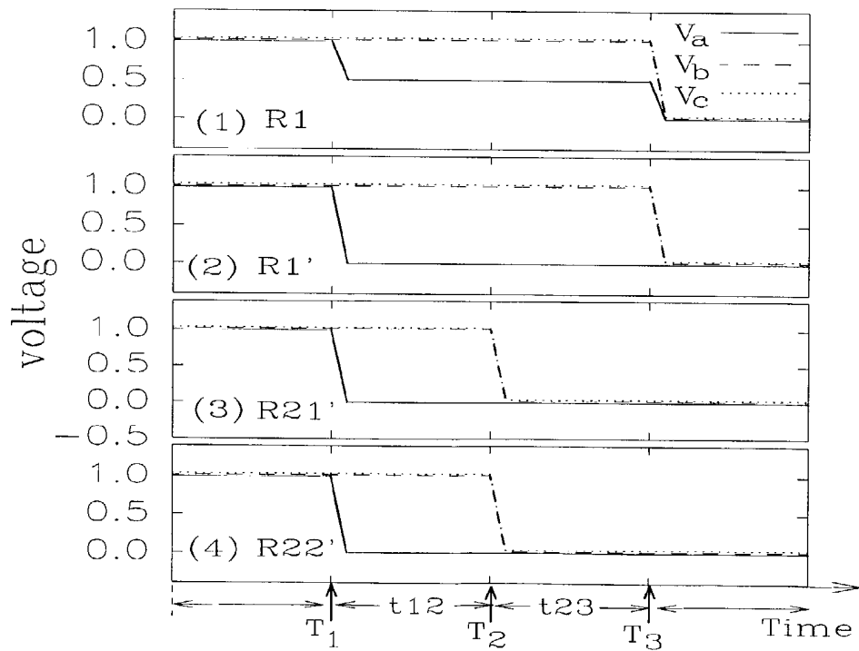
Figure 3b (Fault phase 'a'-e' on Line L1)
