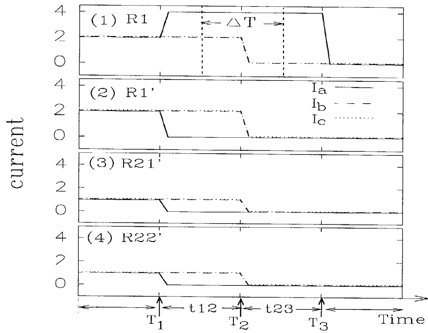
Figure 3a (Fault phase 'a'-e' on Line L1)
