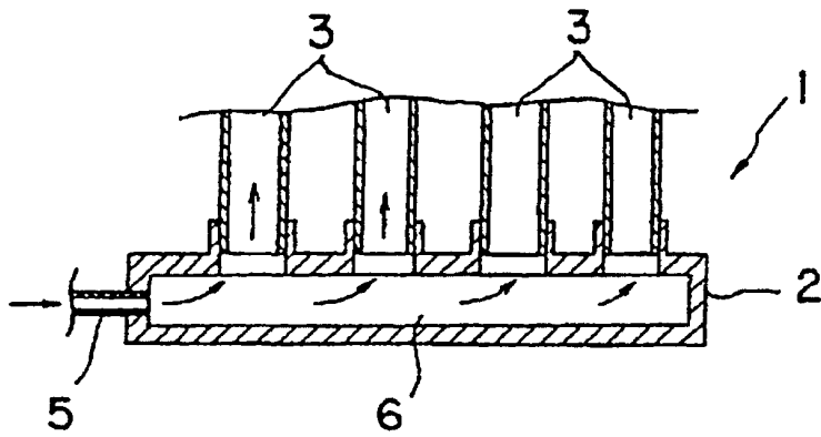
Fig 6 PRIOR ART
