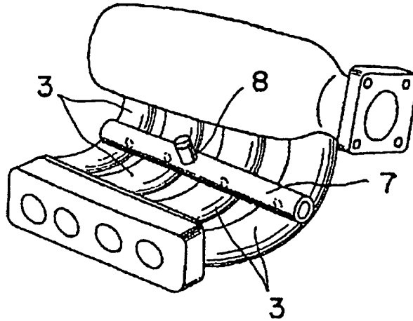
Fig 7 PRIOR ART
