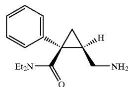
Racemic milnacipran
