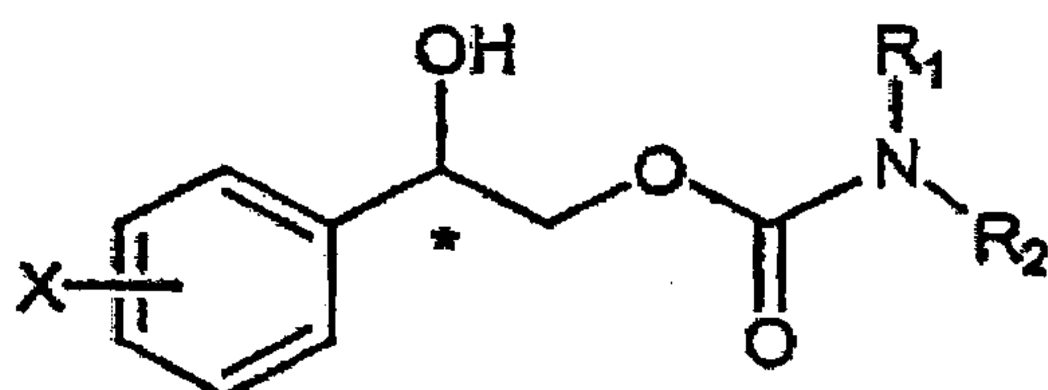
Formula (I)
