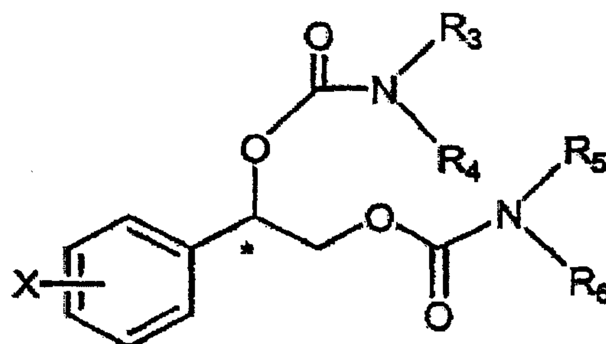
Formula (II)
