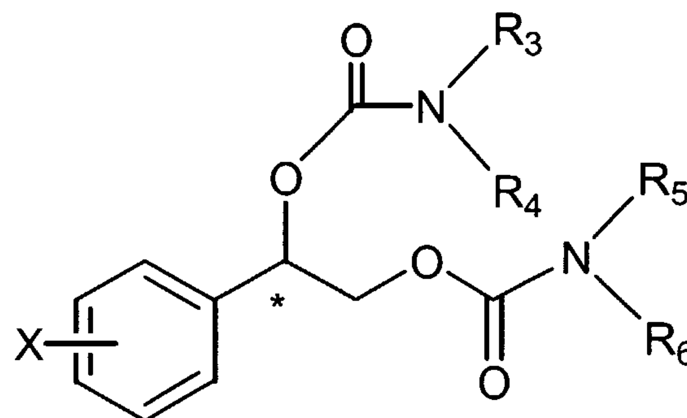
Formula (II)
