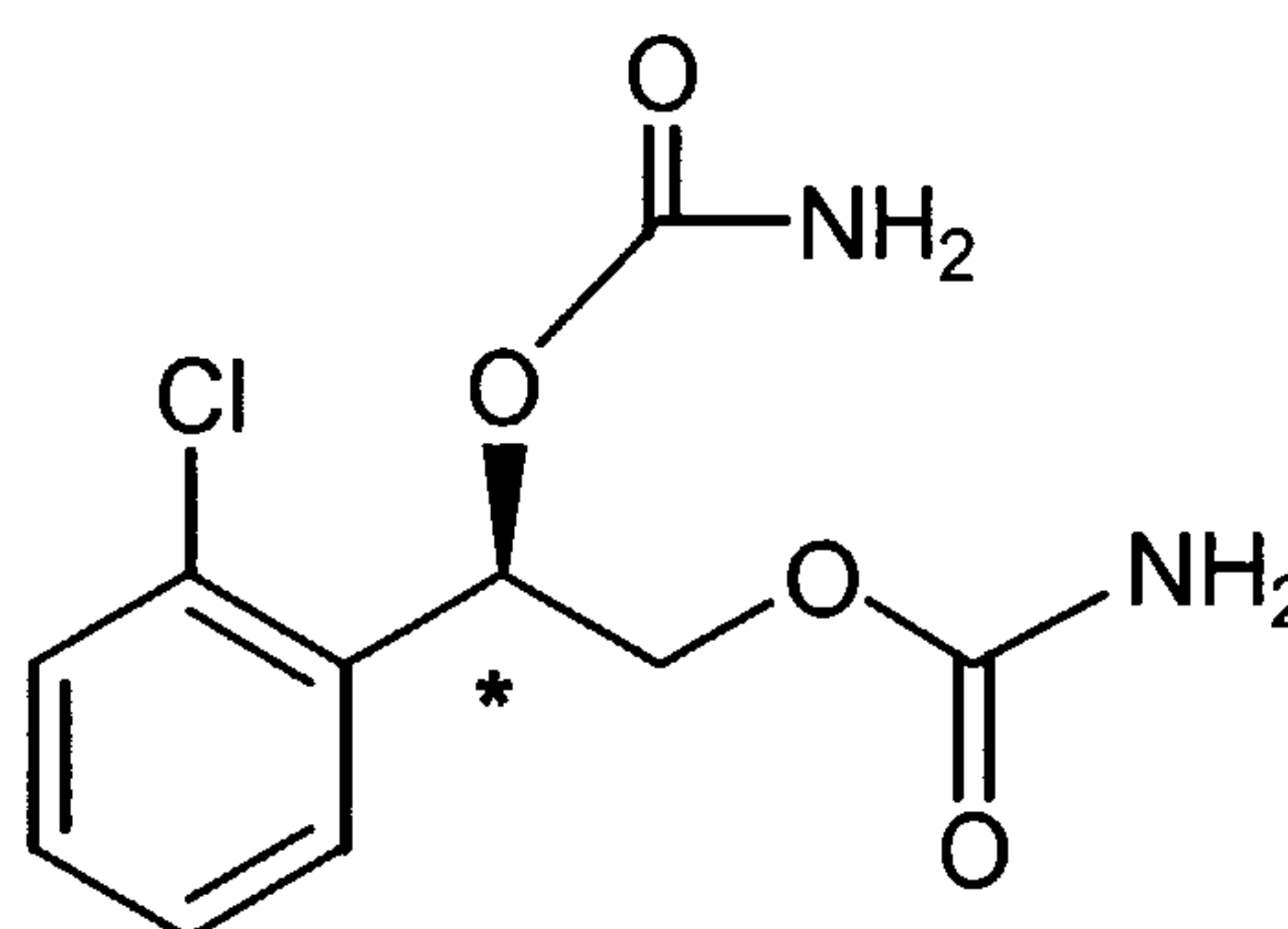
Formula (IIb)
