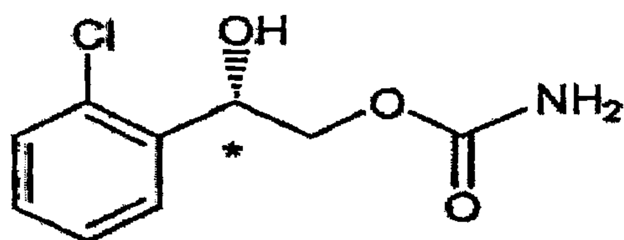
Formula (Ib)
