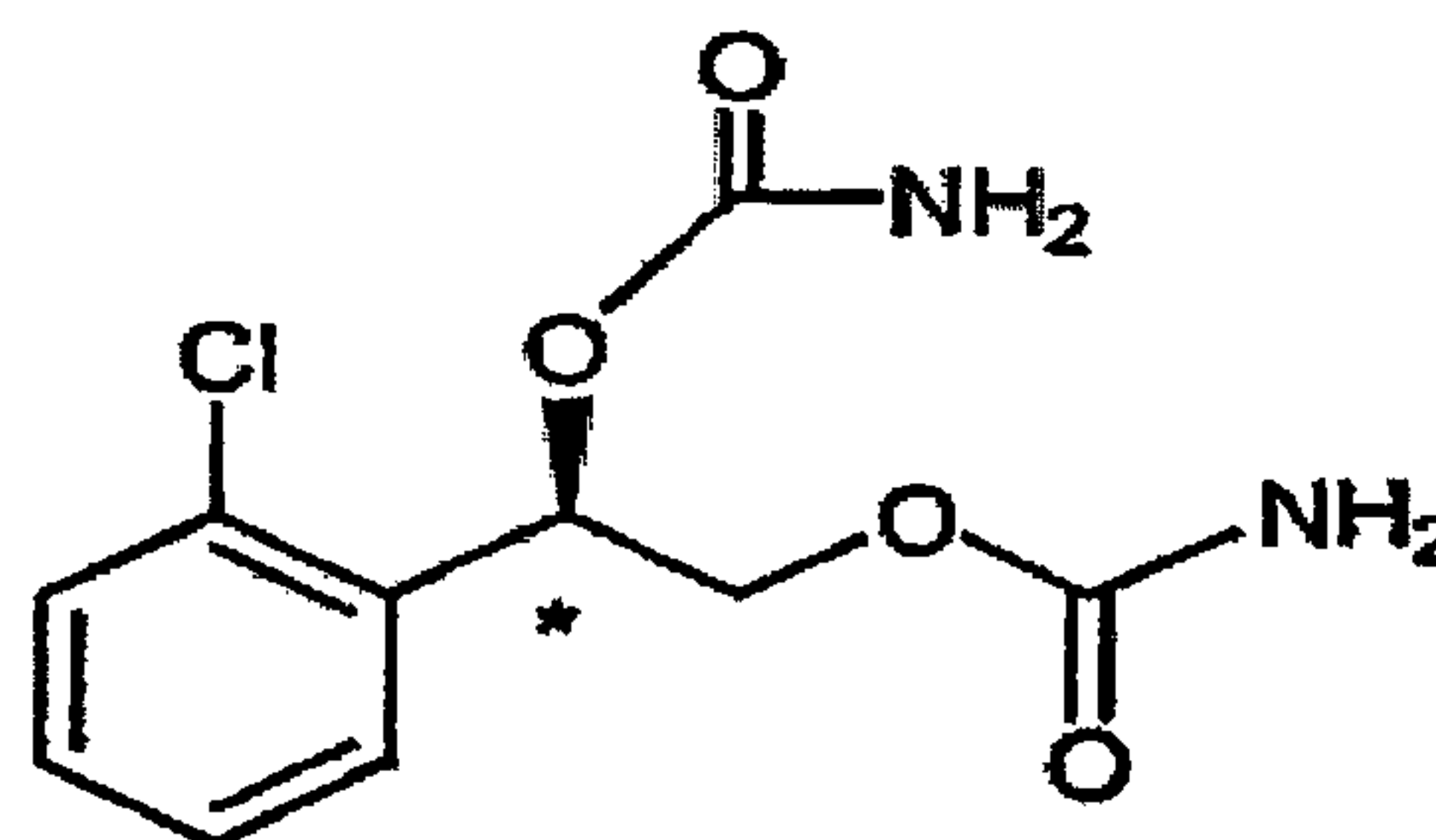
Formula (IIb)
