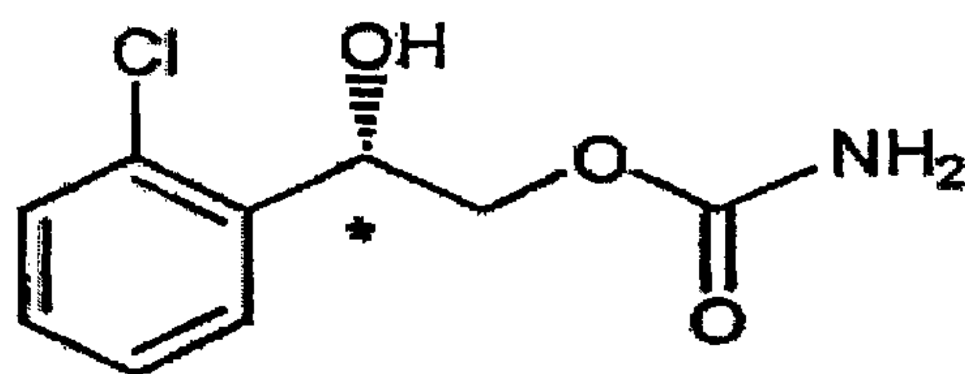
Formula (Ib)
