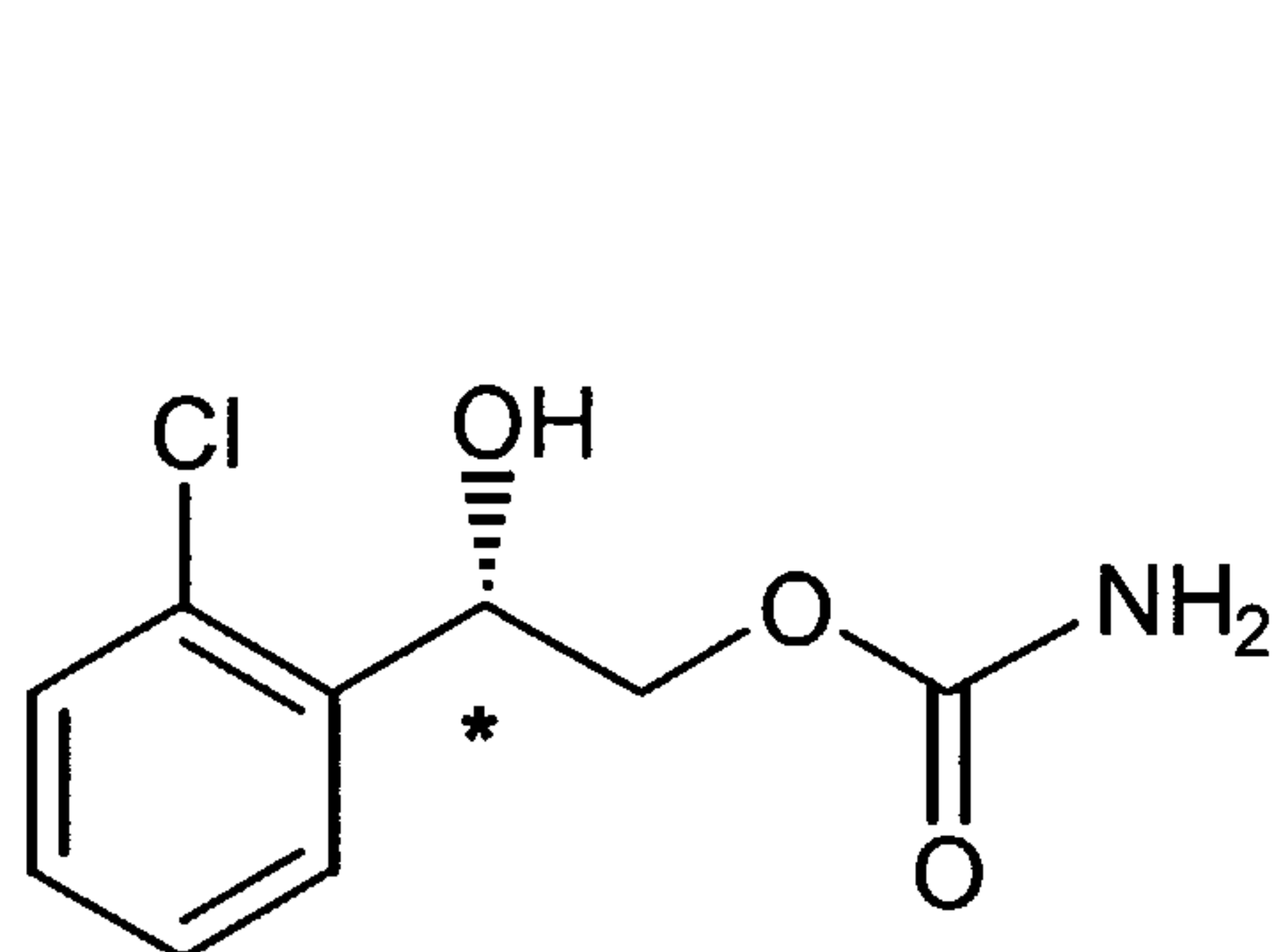
Formula (Ib)
