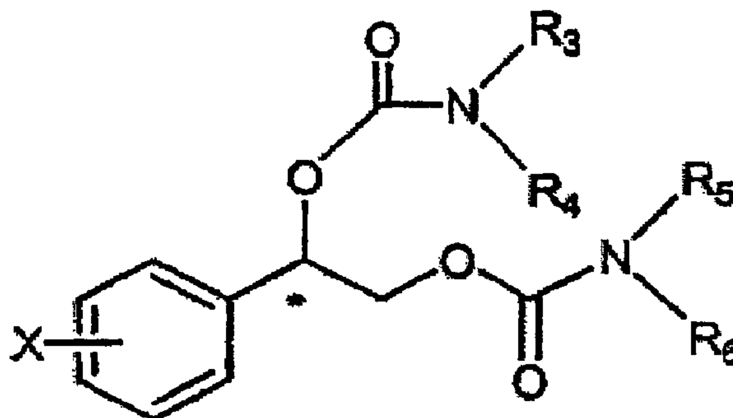
Formula (II)
