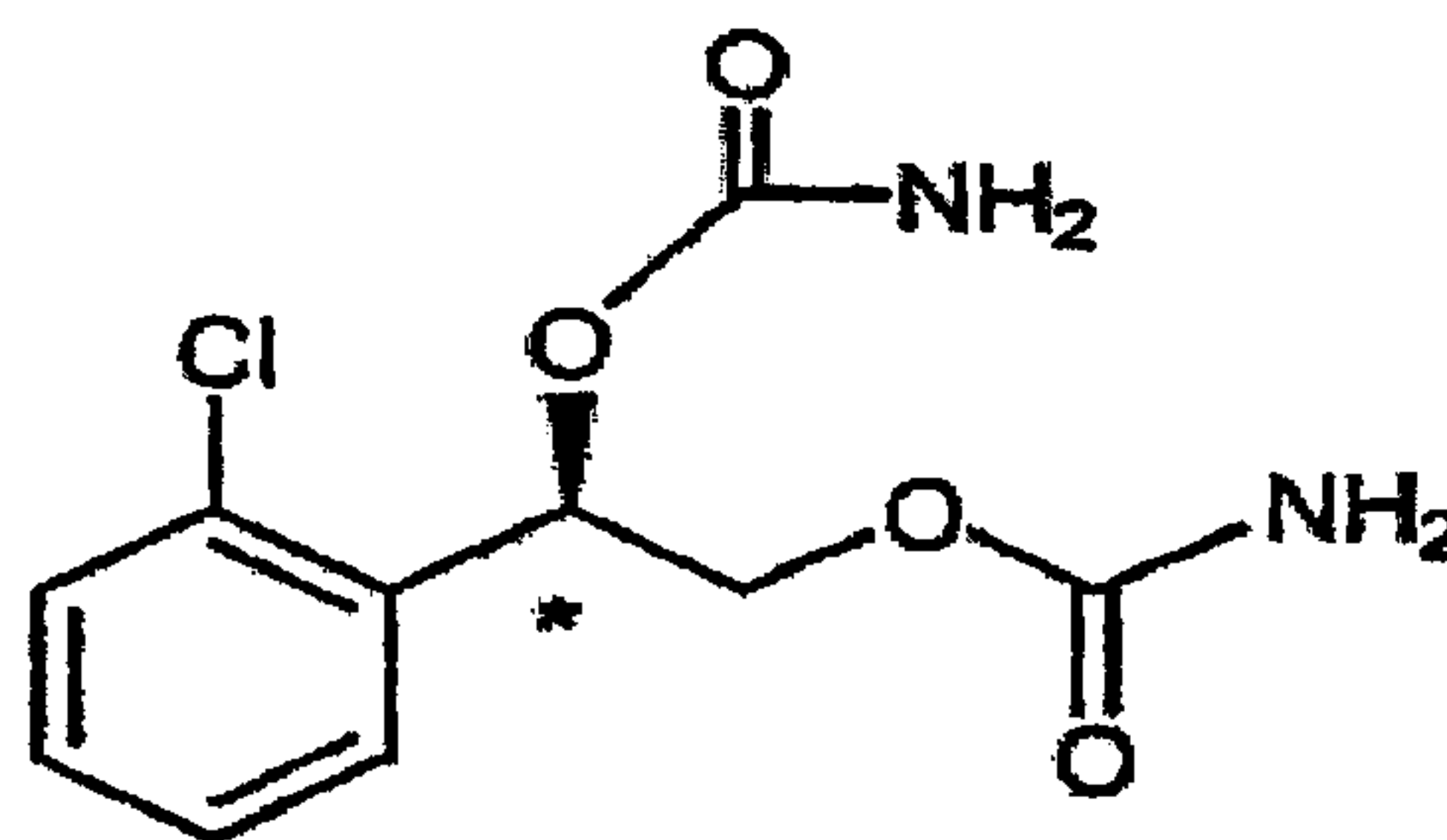
Formula (IIb)
