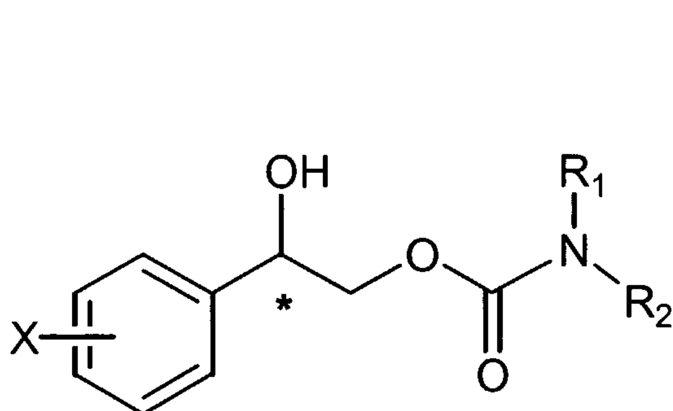
Formula (I)
