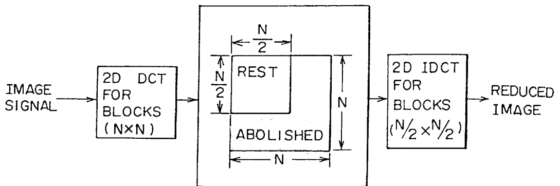
FIG. 59 PRIOR ART
