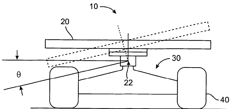
FIG. 3 (Prior Art)
