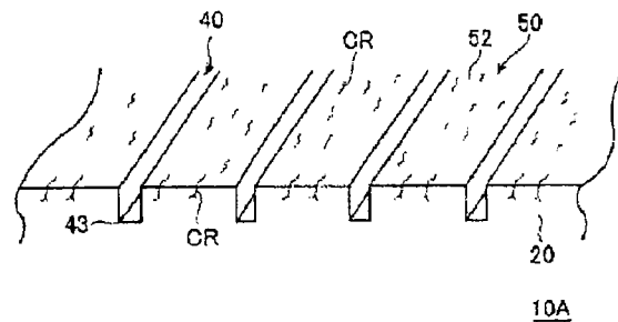
Fig. 6 PRIOR ART
