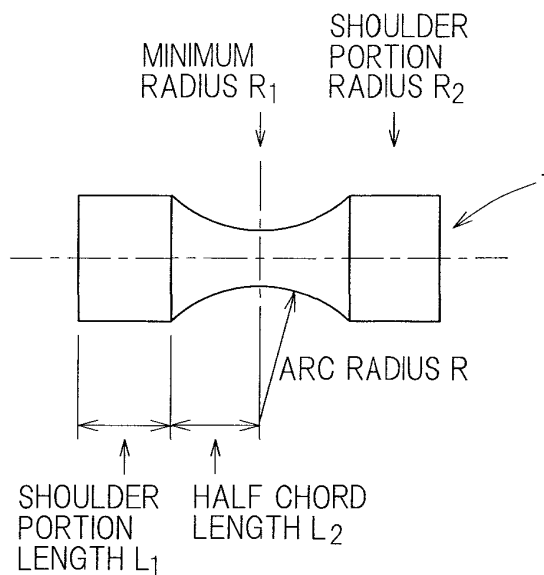
SCHEMATIC DIAGRAM OF TEST PIECE
