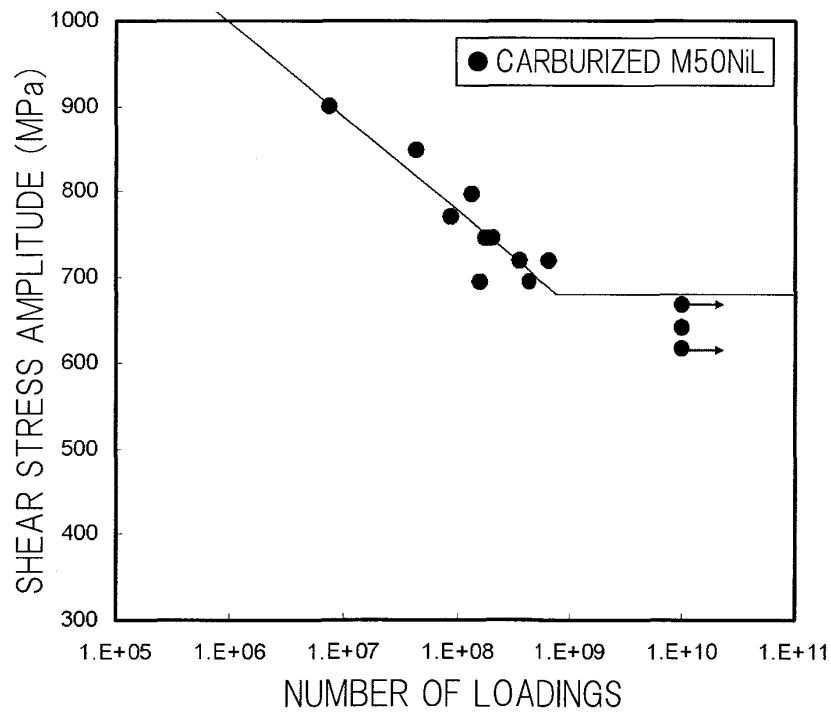
SHEAR FATIGUE PROPERTY OF CARBURIZED M50NiL
