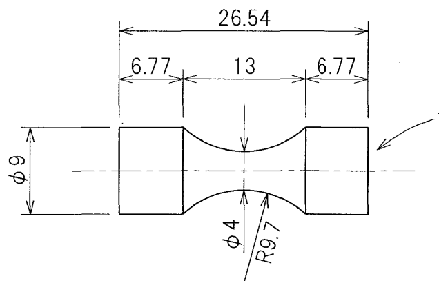
DIAGRAM OF TEST PIECE SUBJECT TO TEST (mm IN UNIT)
