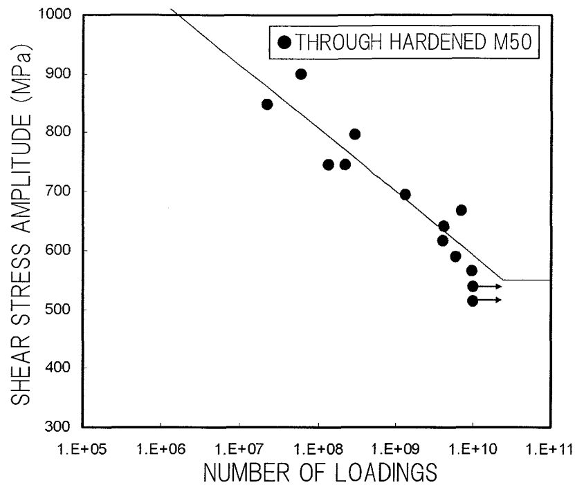
SHEAR FATIGUE PROPERTY OF THROUGH HARDENED M50
