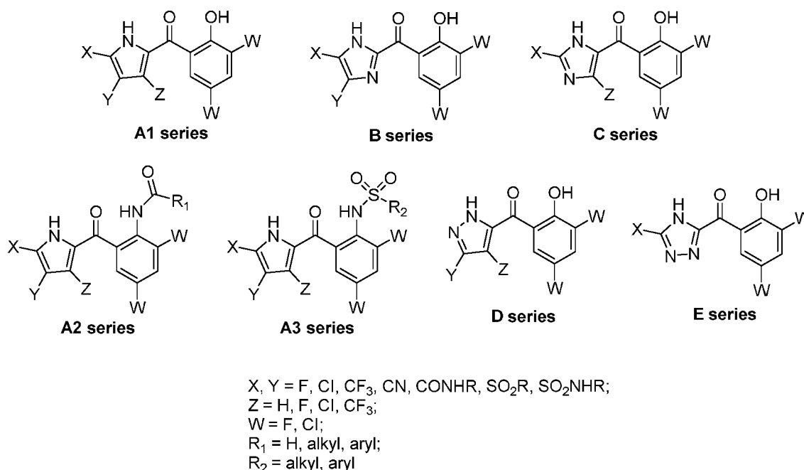
Chart 1. Novel pyrrolomycins and their bioisosteres
