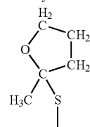
2-methyl tetrahydrofuryl
