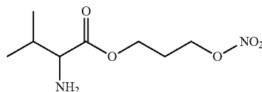
2'-nitrooxypropyl 2-amino-3-methylbutanoate.
