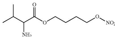
2'-nitrooxybutyl 2-amino-3-methylbutanoate.
