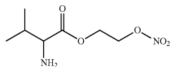
2'-nitrooxyethyl 2-amino-3-methylbutanoate.
