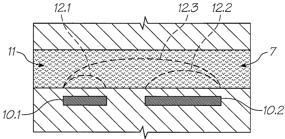
FIG. 52 (PRIOR ART)
