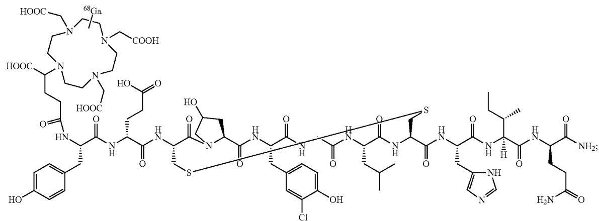
Compound ^{68}\text{Ga} -23
