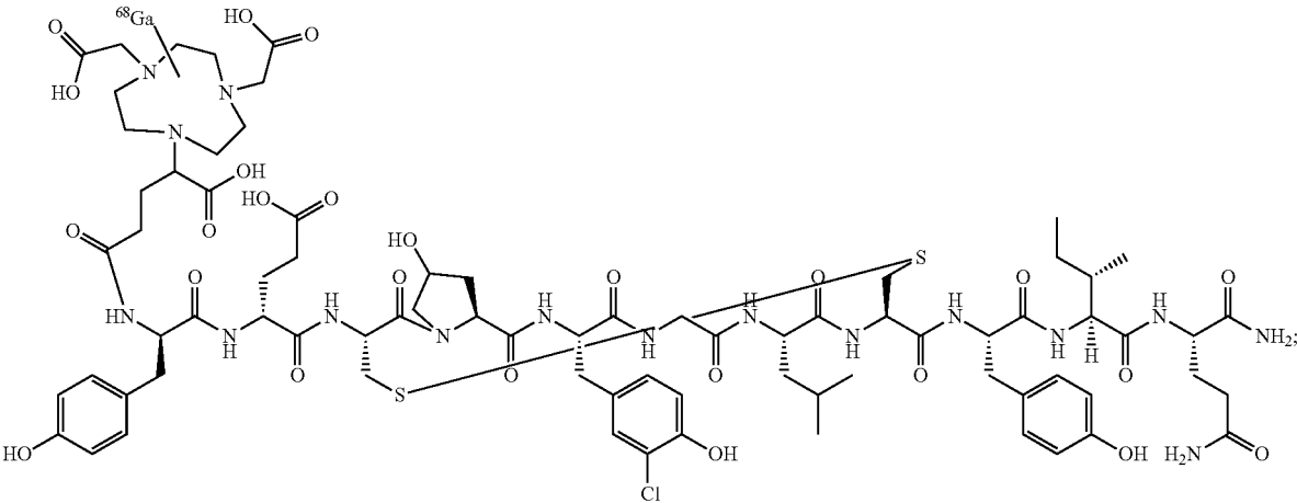
Compound 68 Ga-17
