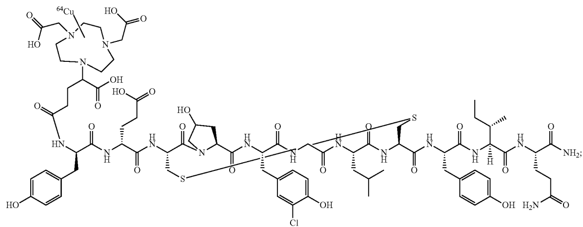
Compound ^{64}\text{Cu} -17
