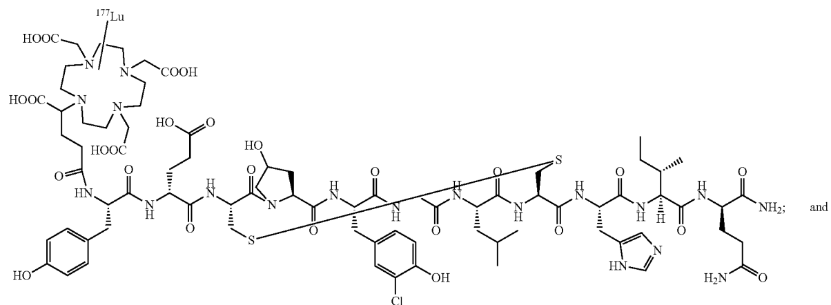
Compound 177 Lu-23
