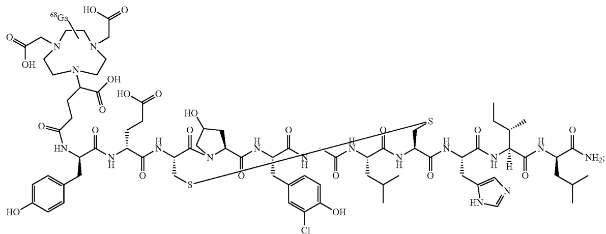
Compound ^{68}\text{Ga} -21
