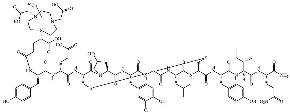
Compound ^{64}\text{Cu} -17
