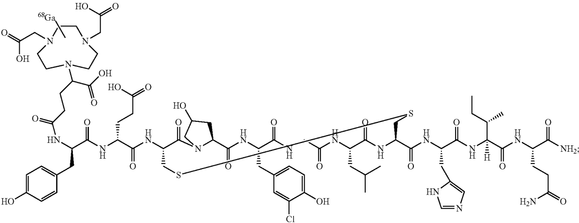
Compound 68 Ga-19
