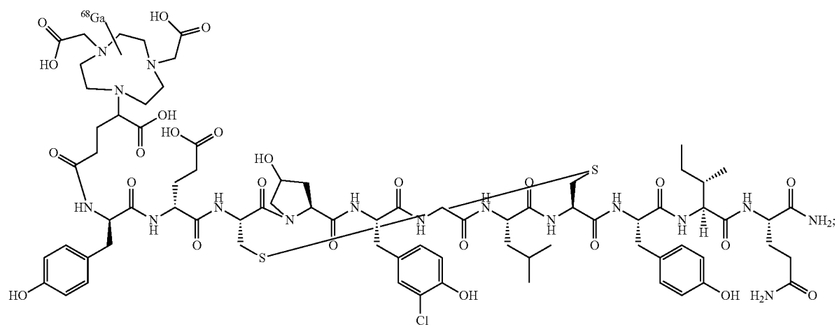
Compound 68 Ga-18
