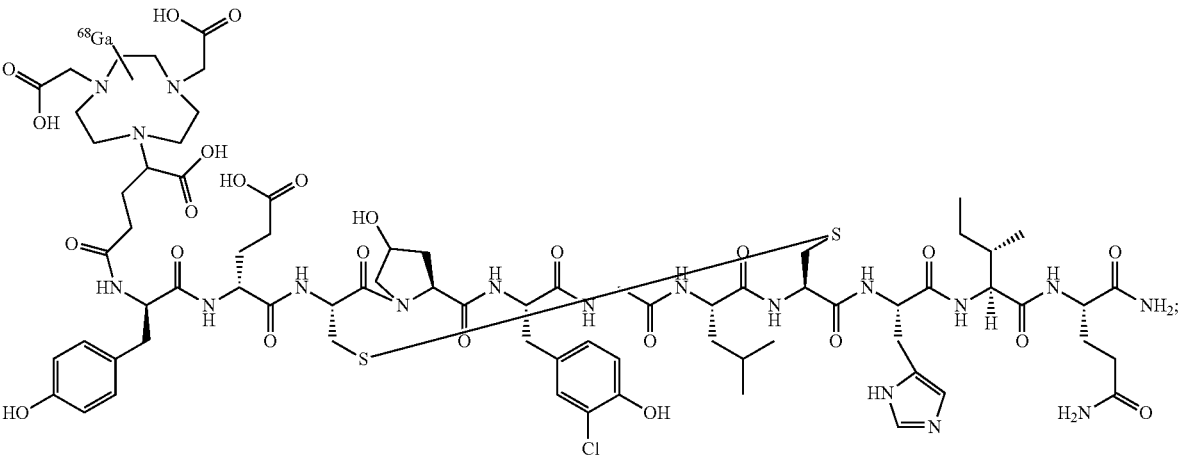
Compound 68 Ga-19
