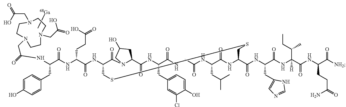
Compound ^{68}\text{Ga} -24
