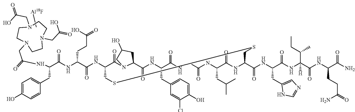
Compound Al 18 F-24
