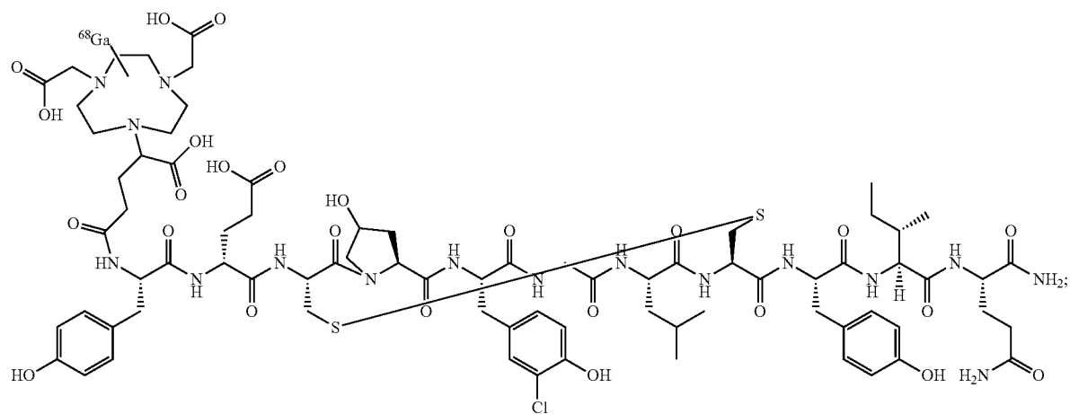
Compound 68 Ga-17
