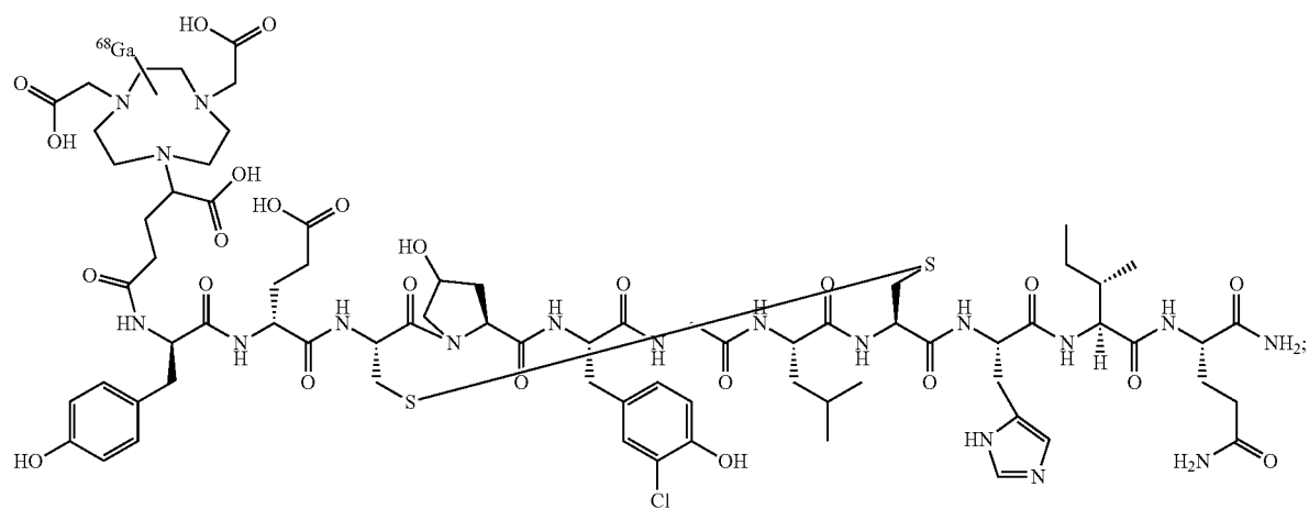
Compound ^{68}\text{Ga} -20
