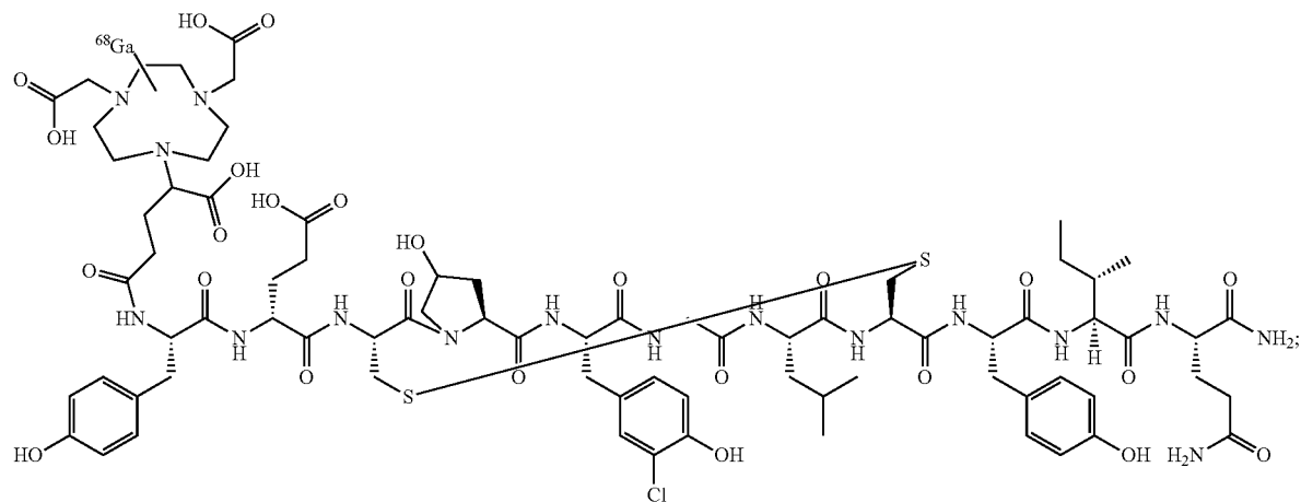
Compound ^{68}\text{Ga} -17
