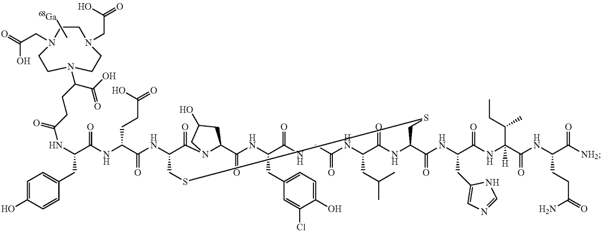
Compound 68 Ga-18
