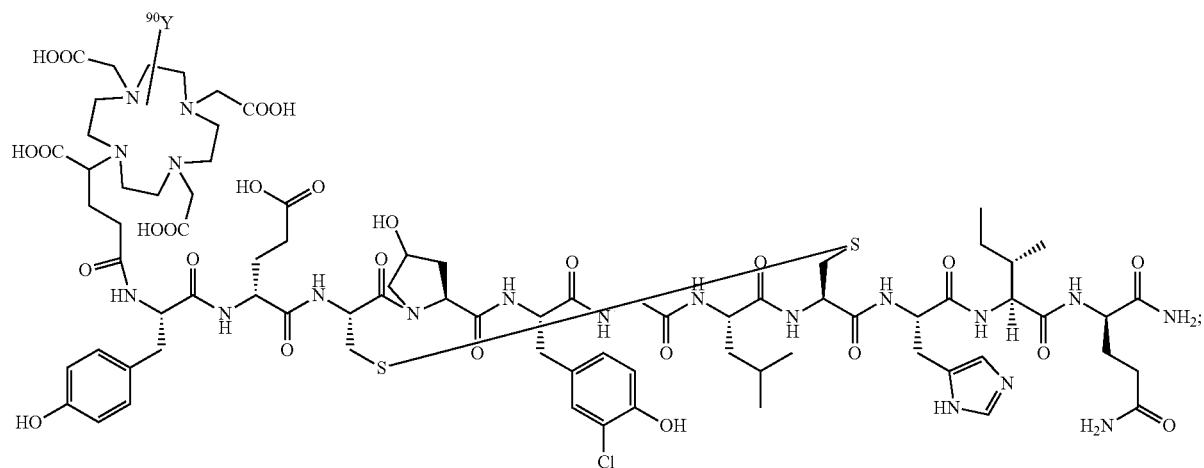
Compound 177 Lu-23
