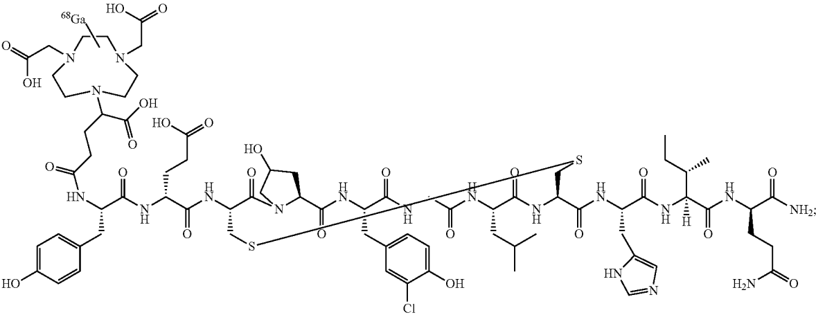
Compound 68 Ga-20
