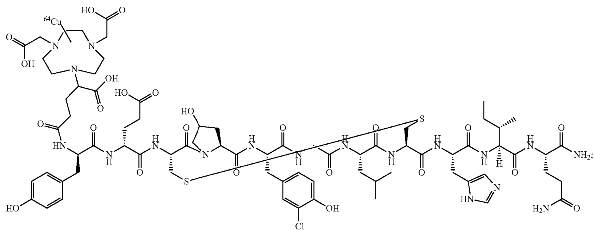
Compound ^{64}\text{Cu} -19
