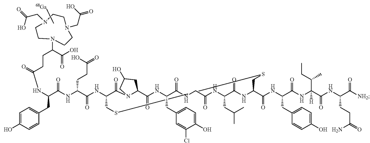
Compound ^{68}\text{Ga} -17
