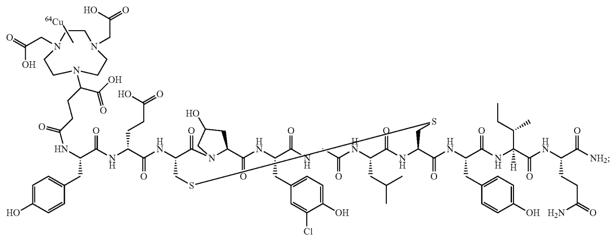
Compound ^{64}\text{Cu} -16
