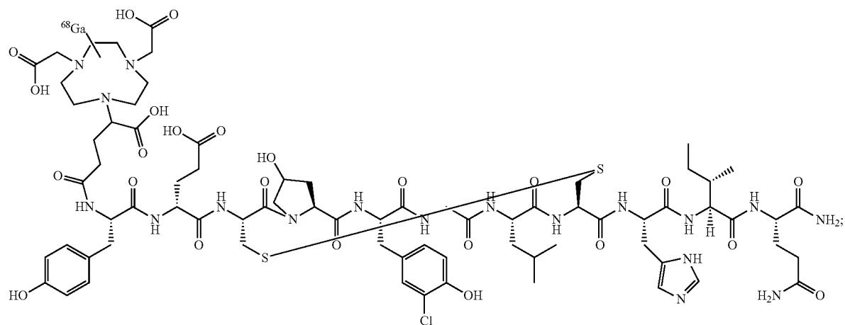
Compound 68 Ga-18
