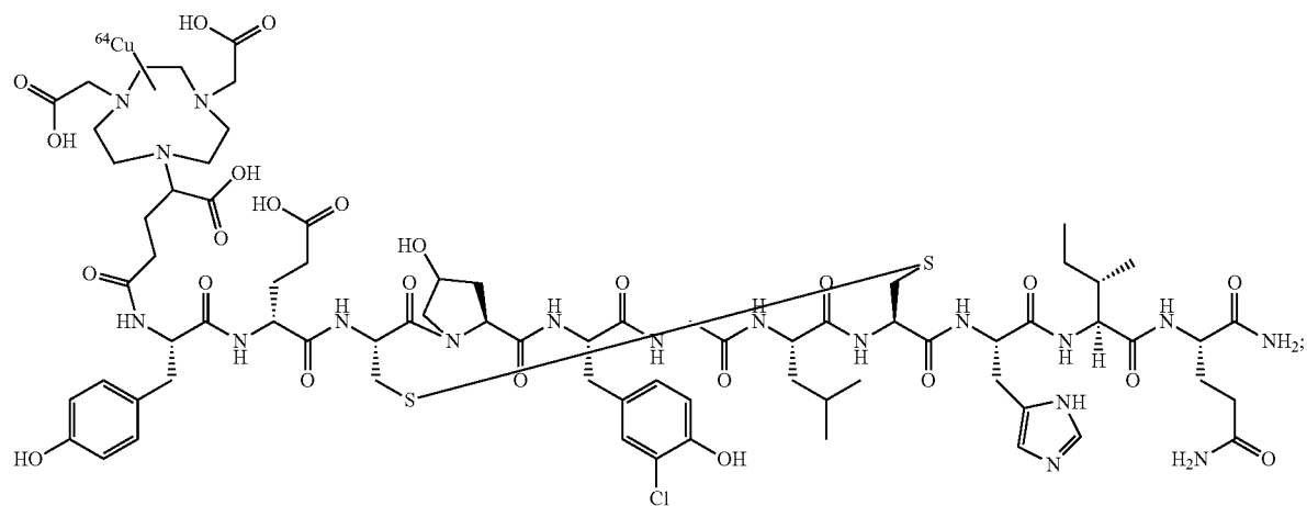
Compound ^{64}\text{Cu} -18
