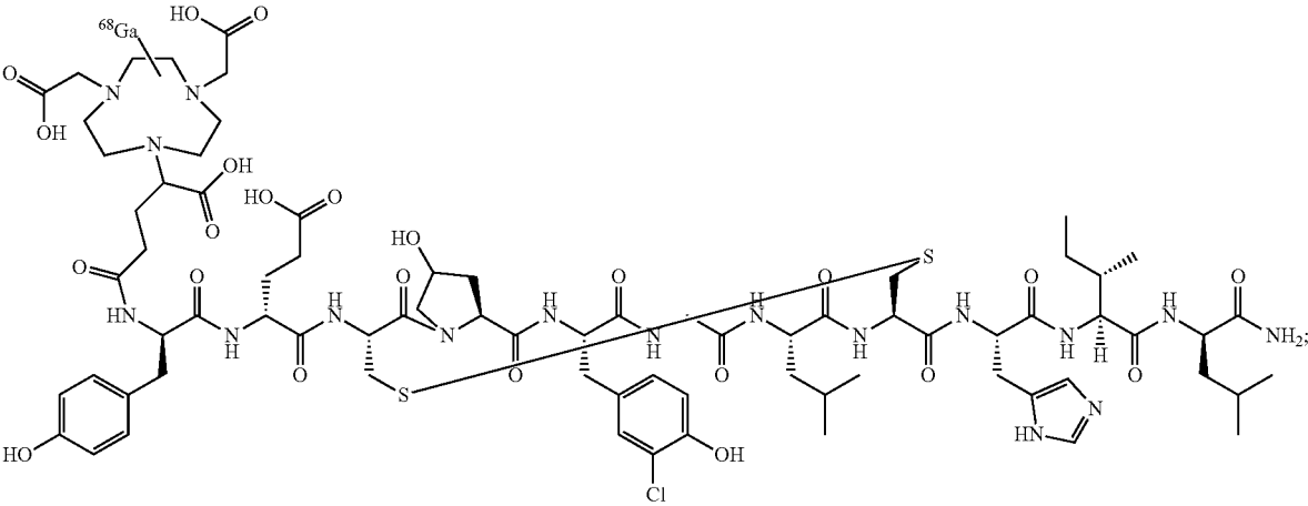
Compound 68 Ga-21
