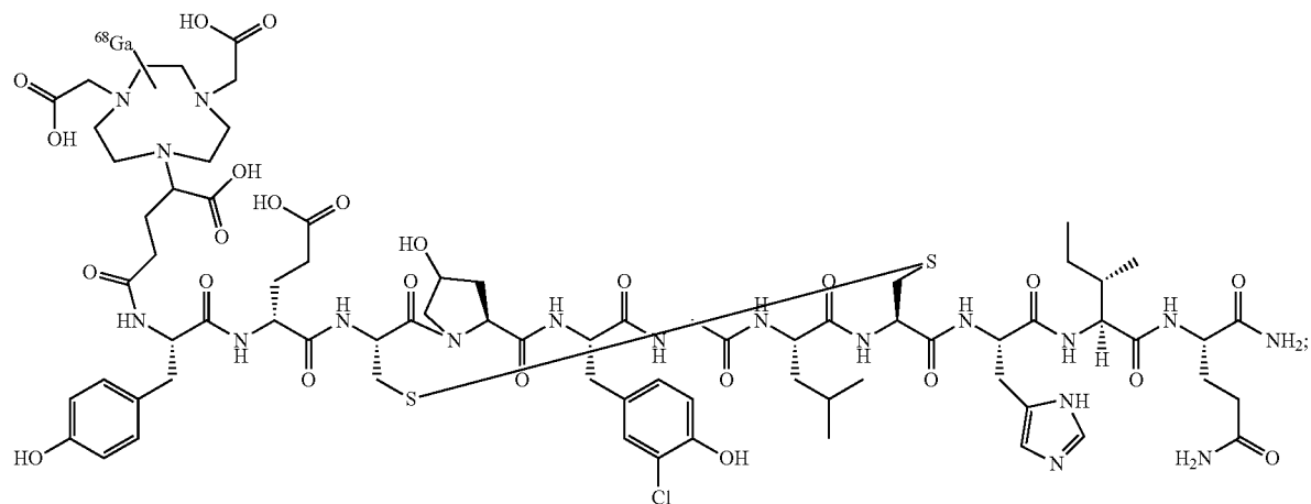
Compound ^{68}\text{Ga} -18
