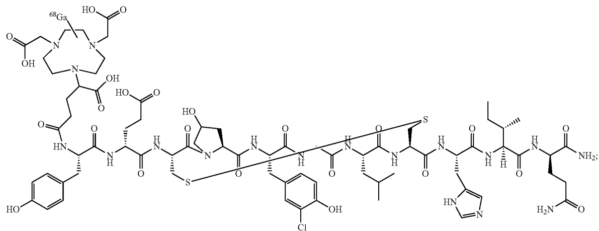
Compound ^{68}\text{Ga} -20
