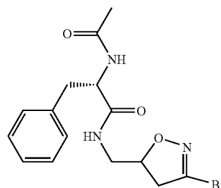
(S)-2-Acetylamino-N-(3-bromo-4,5-dihydro-isoxazol-5-ylmethyl)-3-phenyl-propionamide
