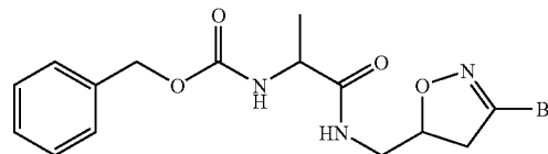
{(S)-1-[(3-Bromo-4,5-dihydro-isoxazol-5-ylmethyl)-carbamoyl]-ethyl}-carbamamic acid benzyl ester
