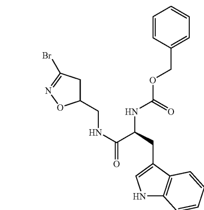
[(S)-1-[(3-Bromo-4,5-dihydro-isoxazol-5-ylmethyl)-carbamoyl]-2-(1H-indol-3-yl)-ethyl]-carbamic acid benzyl ester
