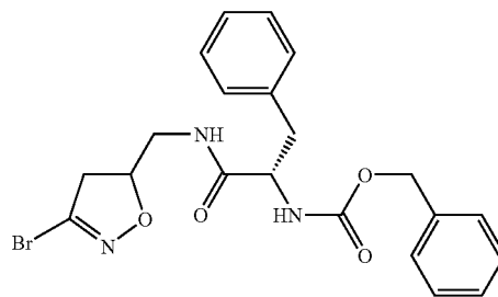
{(S)-1-[(3-Bromo-4,5-dihydro-isoxazol-5-ylmethyl)-carbamoyl]-2-phenyl-ethyl}-carbamic acid benzyl ester
