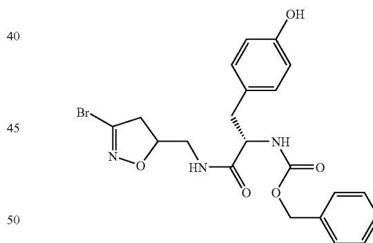
[(S)-1-[(3-Bromo-4,5-dihydro-isoxazol-5-ylmethyl)-methyl-carbamoyl]-2-(4-hydroxy-phenyl)-ethyl]-carbamic acid benzyl ester
