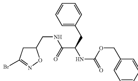
{(R)-1-[(3-Bromo-4,5-dihydro-isoxazol-5-ylmethyl)-carbamoyl]-2-phenyl-ethyl}-carbamamic acid benzyl ester
