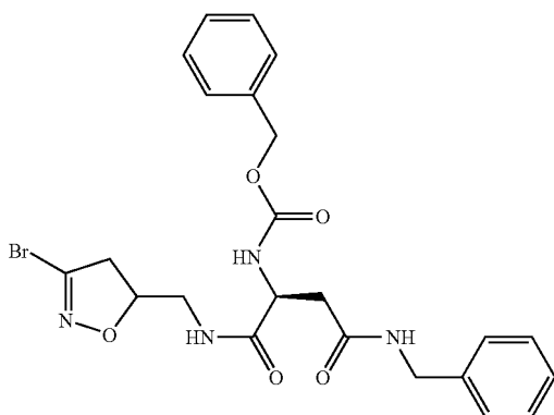
{(S)-2-Benzylcarbamoyl-1-[(3-bromo-4,5-dihydro-isoxazol-5-ylmethyl)-carbamoyl]-ethyl}-carbamic acid benzyl ester
