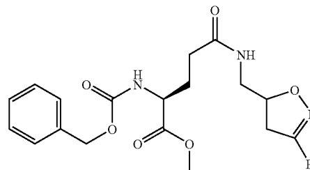
(S)-2-Benzyloxycarbonylamino-4-[(3-bromo-4,5-dihydro-isoxazol-5-ylmethyl)-carbamoyl]-butyric acid methyl ester
