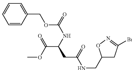
(S)-2-Benzyloxycarbonylamino-N-(3-bromo-4,5-dihydro-isoxazol-5-ylmethyl)-succinamic acid methyl ester
