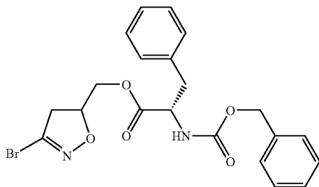
(S)-2-Benzyloxycarbonylamino-3-phenyl-propionic acid 3-bromo-4,5-dihydro-isoxazol-5-ylmethyl ester
