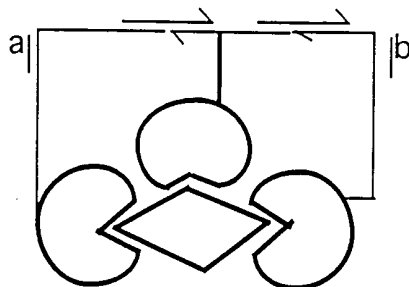
Figure 9. Requirement of two ligation events, using three binding moieties. Amplification primer sites a and b.
