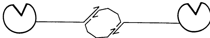
Figure 6. Priming of rolling circle amplification by a proximal oligonucleotide
