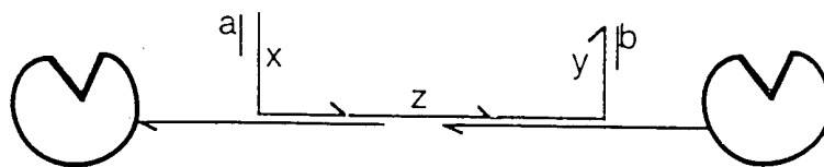
Figure 4. Ligation of supplementary oligonucleotides, x and y, to the proximity-probe-hybridisation oligonucleotide z. Amplification primer sites a and b.
