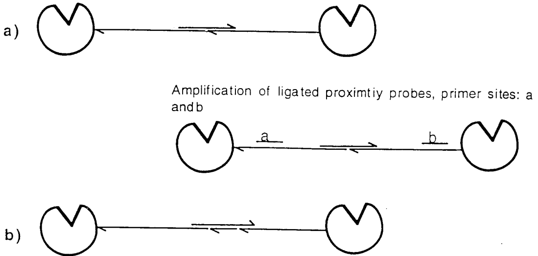
Figure 2. Template promoted ligation variants
