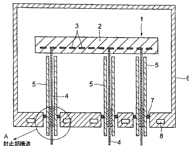
A...SEALING STRUCTURE
