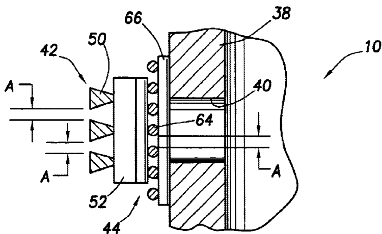
FIG.5 (PRIOR ART)
