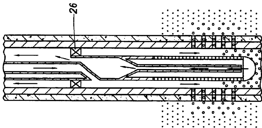
FIG. 3c (PRIOR ART)
