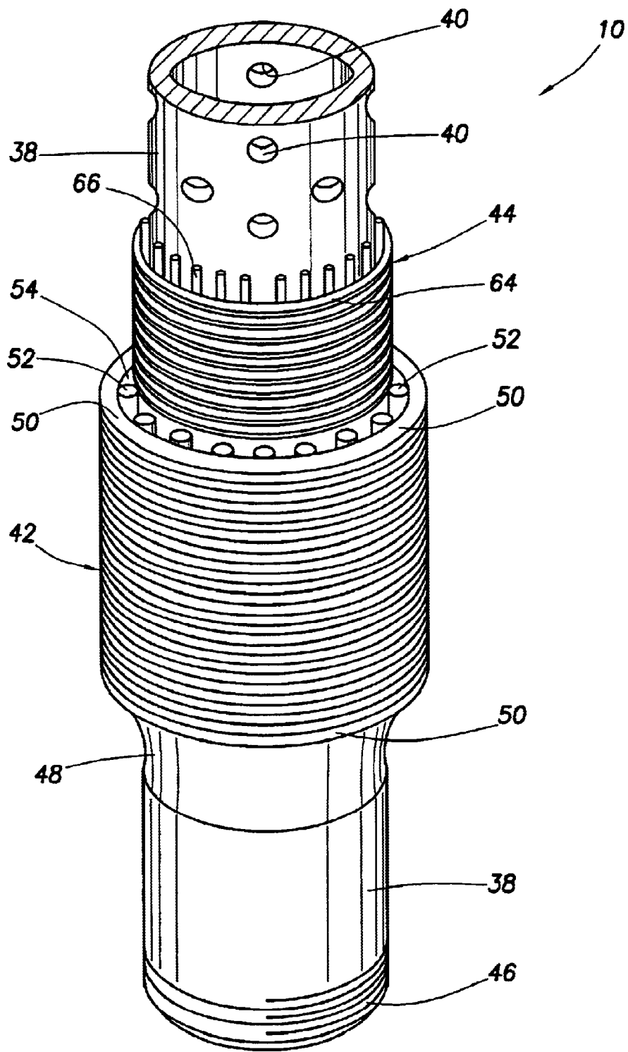
FIG. 4 (PRIOR ART)
