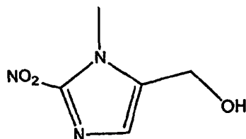
N-1-methyl-2-nitro-5-hydroxymethyl imidazole
