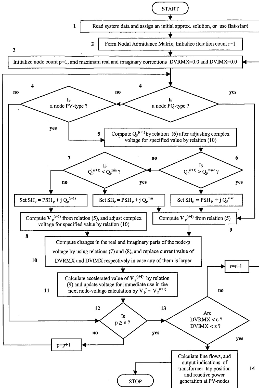
Fig. 1a: Prior Art: flow-chart of Gauss-Seidel Loadflow Algorithm-1a
