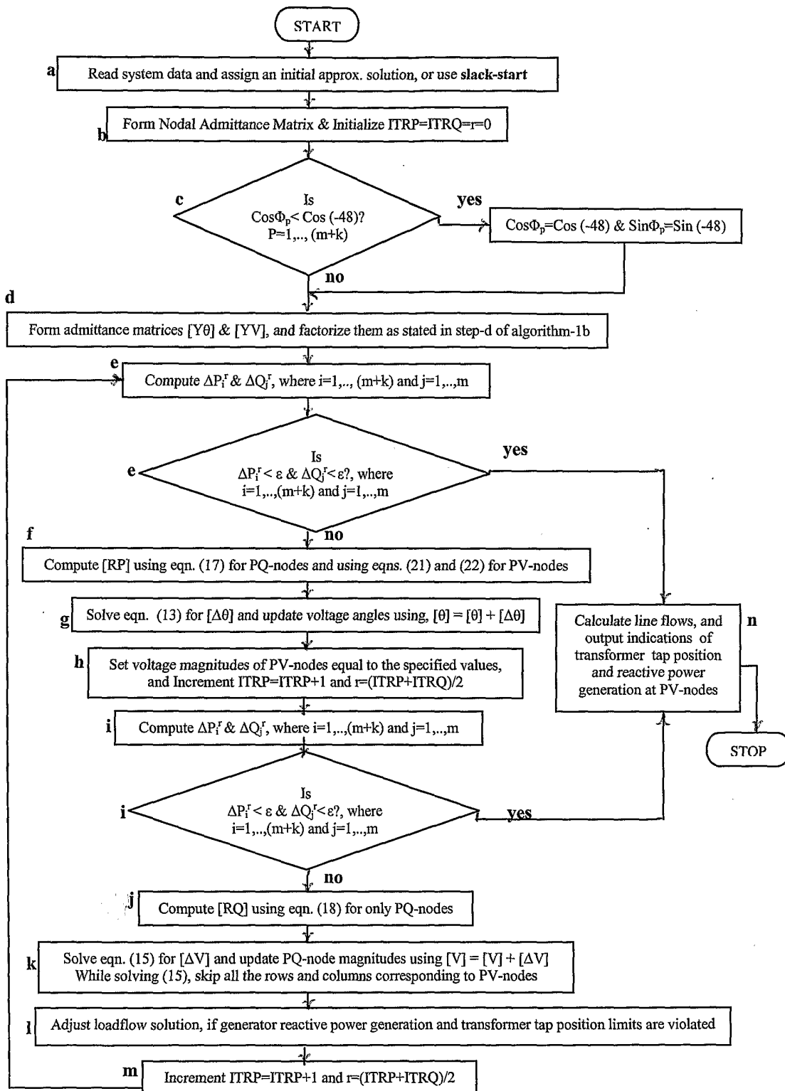
Fig.1b: Prior art: Flow-chart of SSDL solution algorithm-1b
