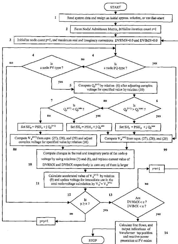
Invention: flow-chart of Gauss-Seidel-Patel Loadflow Algorithm-2a
