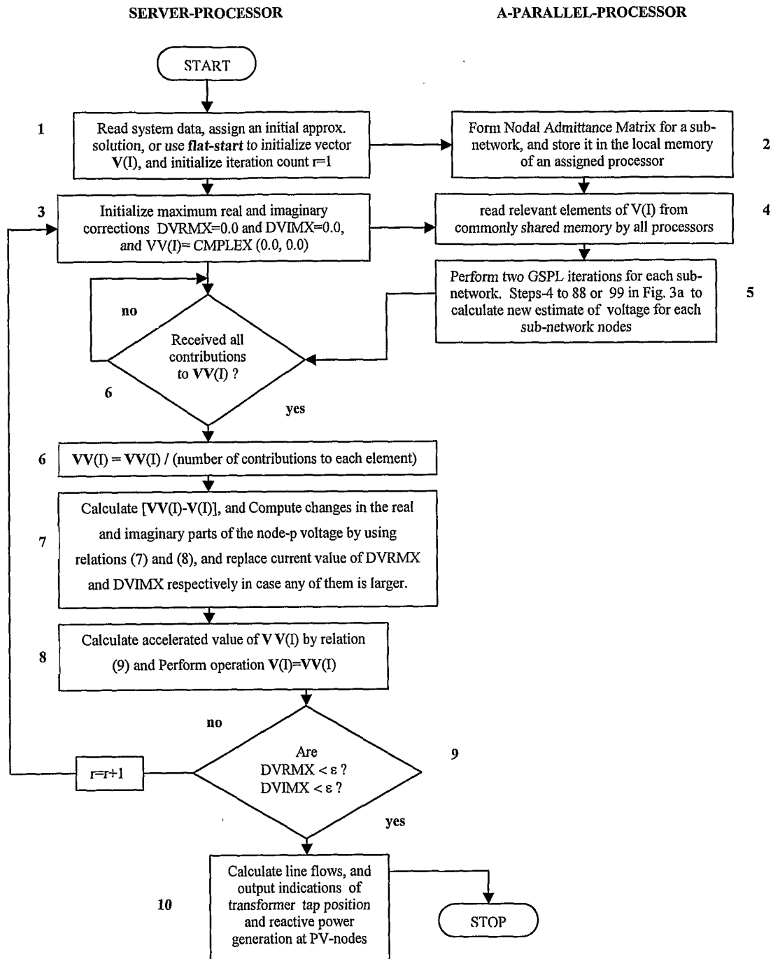
Fig. 3b: Invention: flow-chart of Parallel-Gauss-Seidel-Patel Loadflow Algorithm-2b
