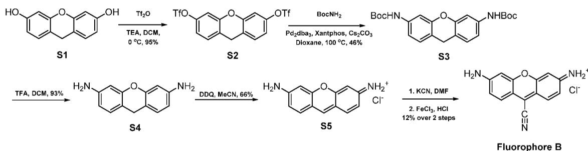
Scheme S1 Synthetic route of Fluorophore B.
