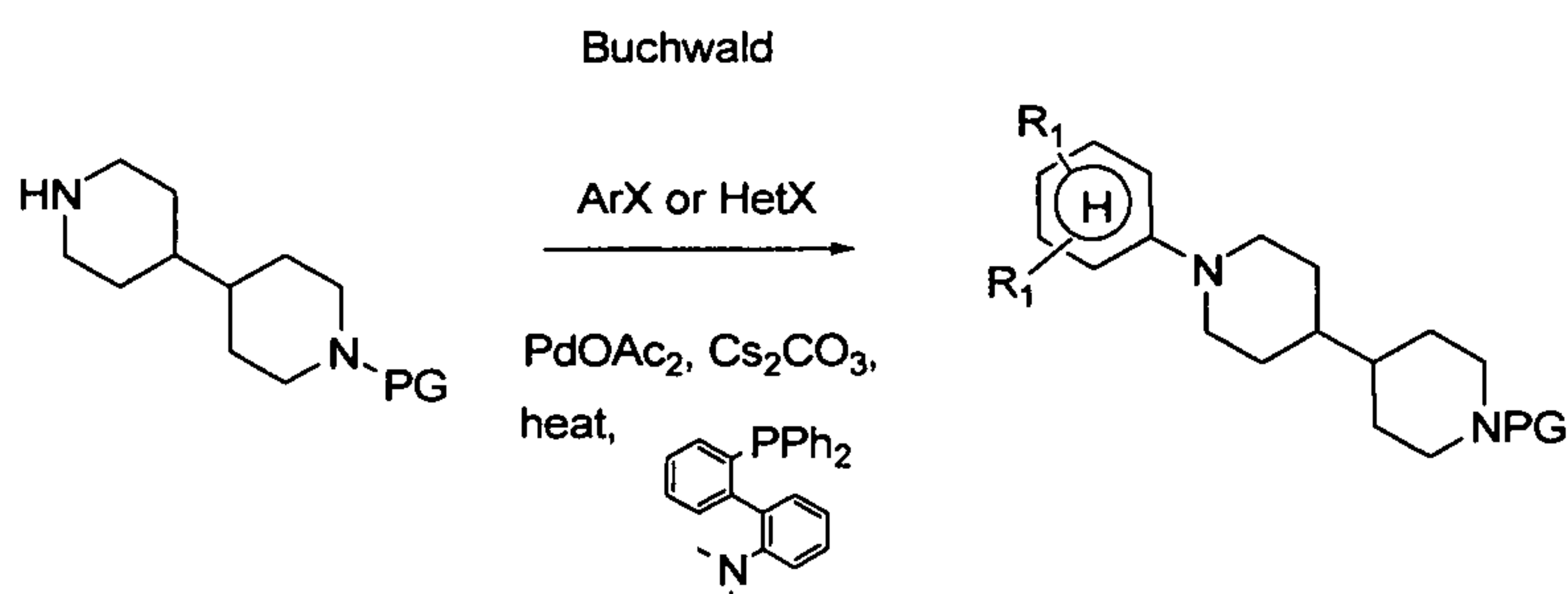
Scheme 3
