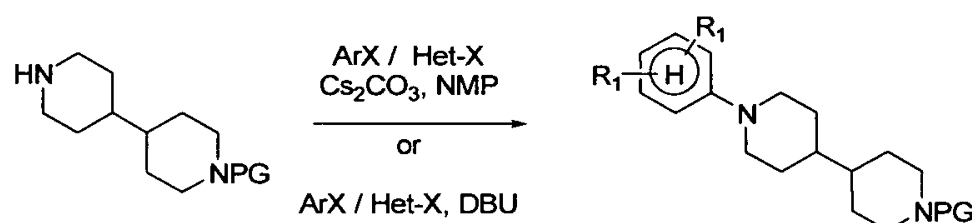
Scheme 2
