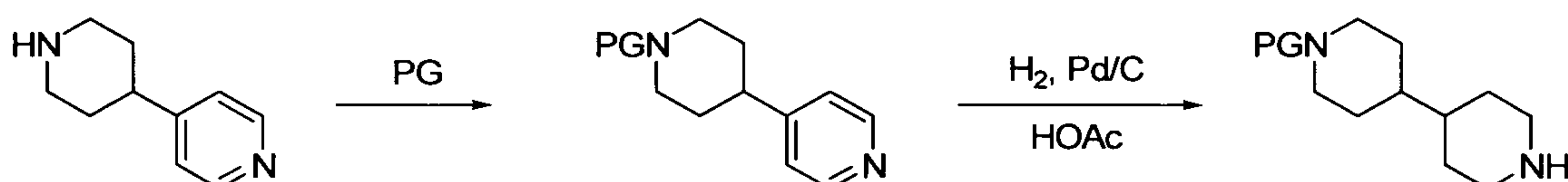
Scheme 1
