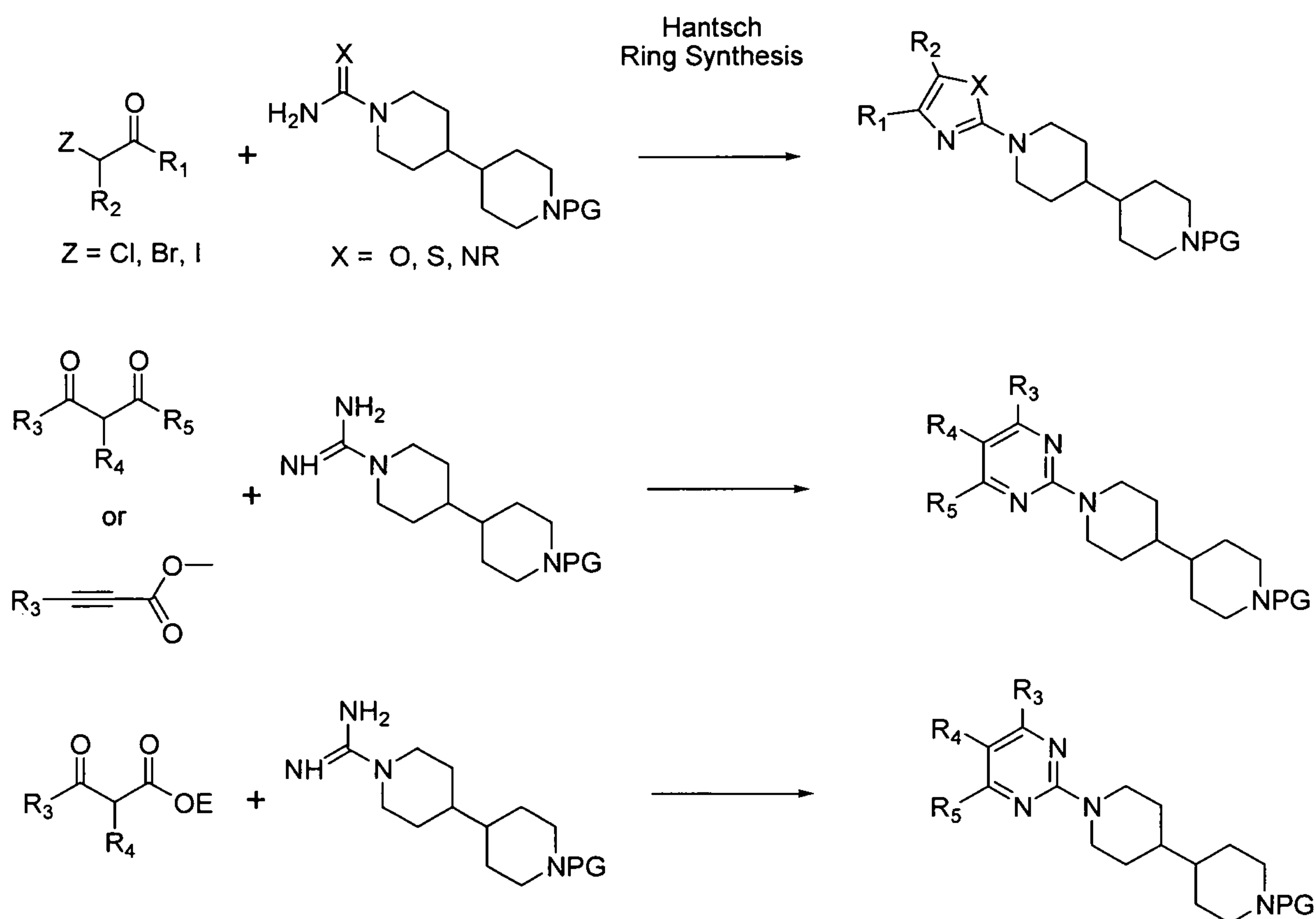
Scheme 4
