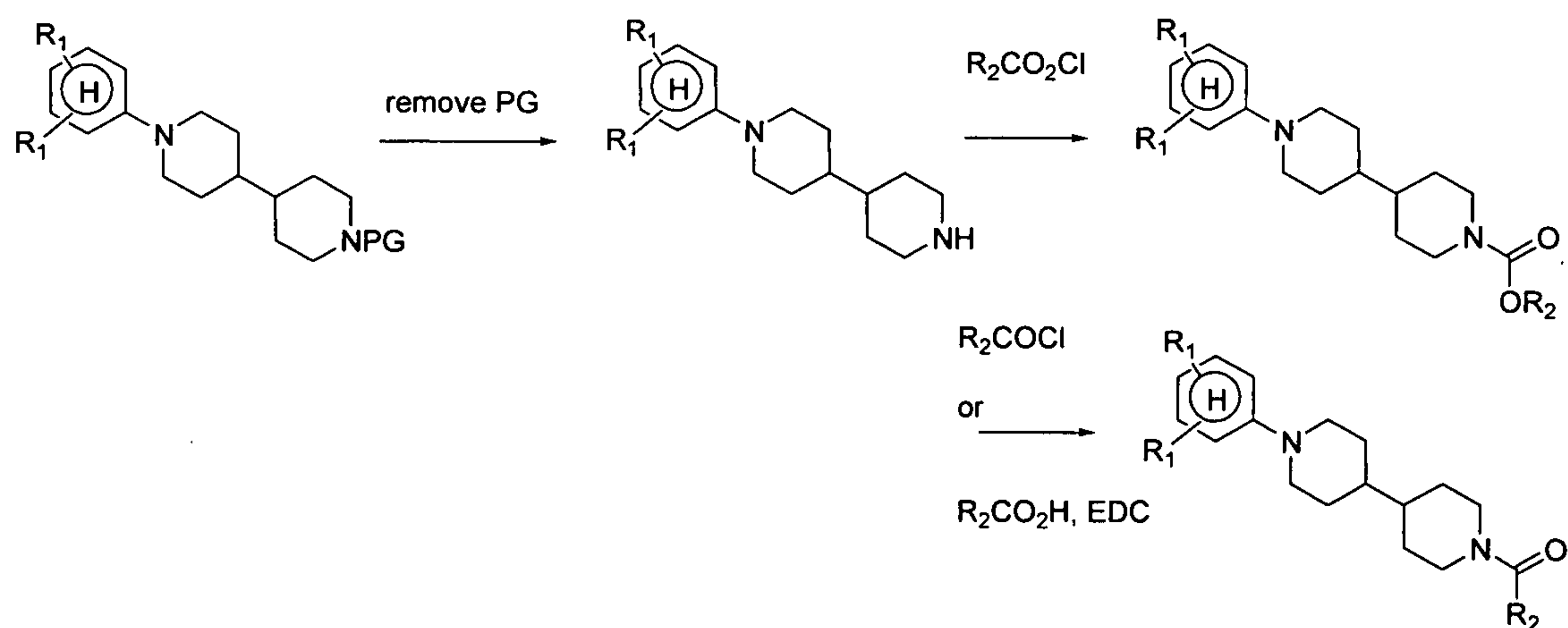
Scheme 6
