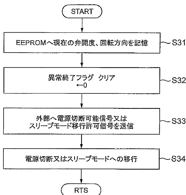
Fig. 8: S31 Store current valve opening degree and rotating direction in EEPROM S32 Clear abnormal termination flag ← 0 S33 Transmit, to outside, signal allowing shut-off or signal permitting transition to sleep mode S34 Shut-off or transition to sleep mode
