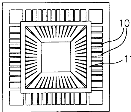
FIG. 2 CONVENTIONAL ART
