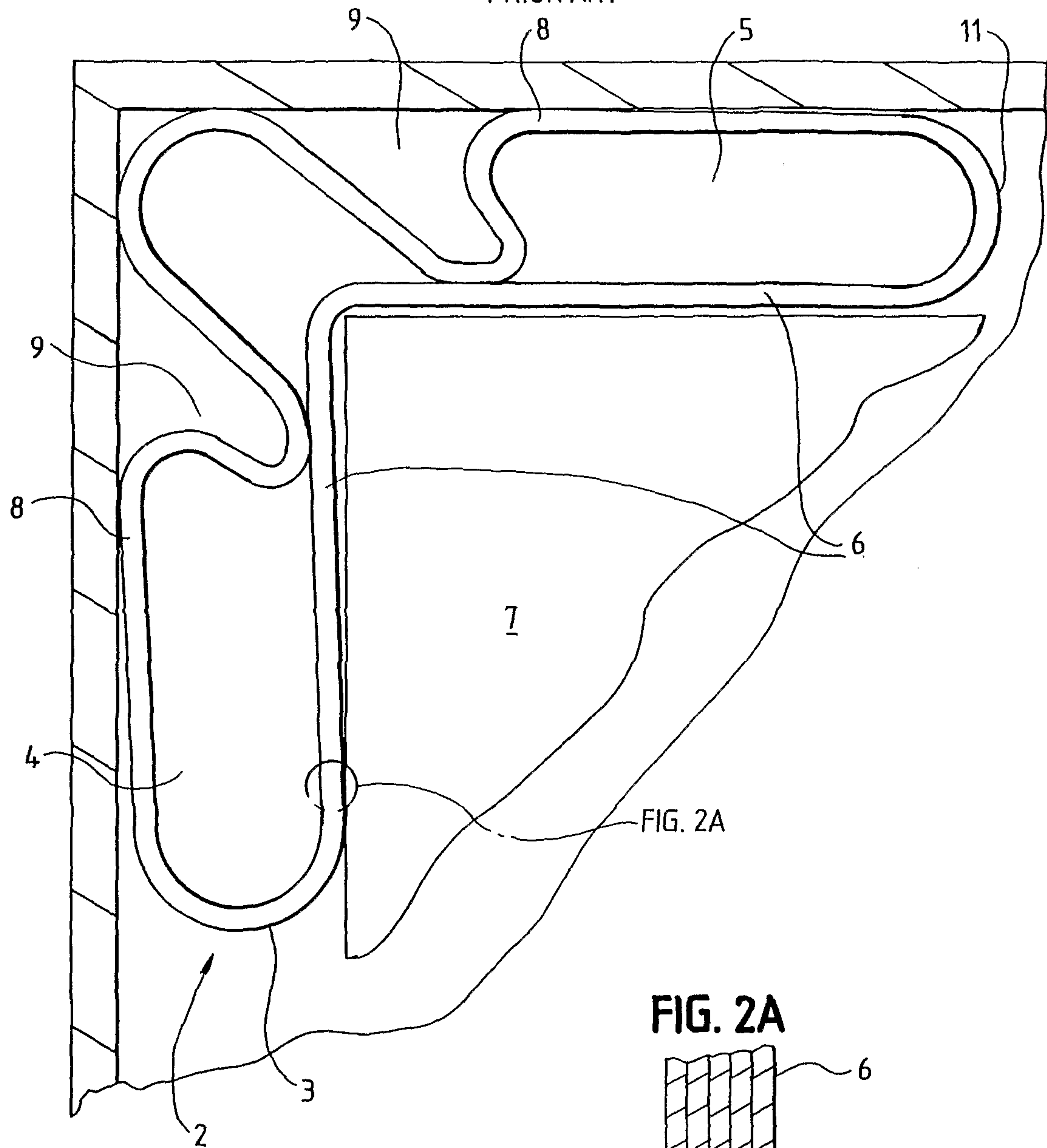
FIG. 2 PRIOR ART
