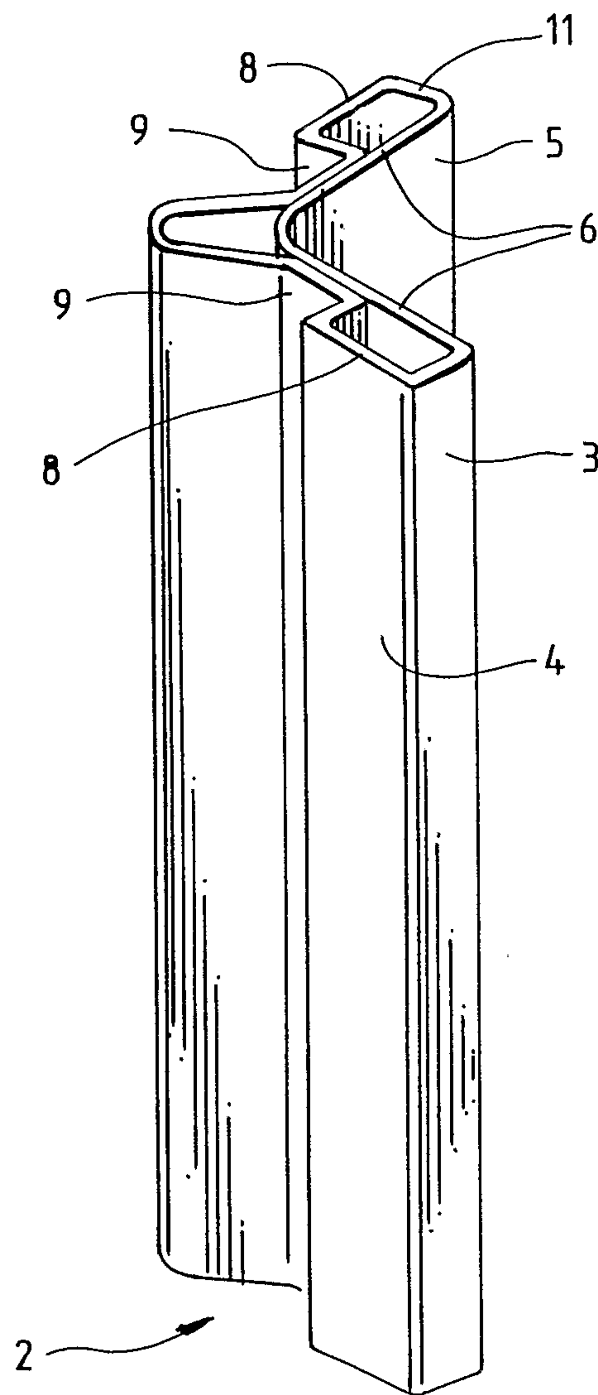
FIG. 1 PRIOR ART
