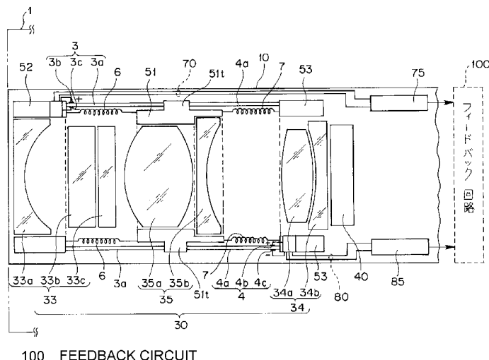
100 FEEDBACK CIRCUIT
