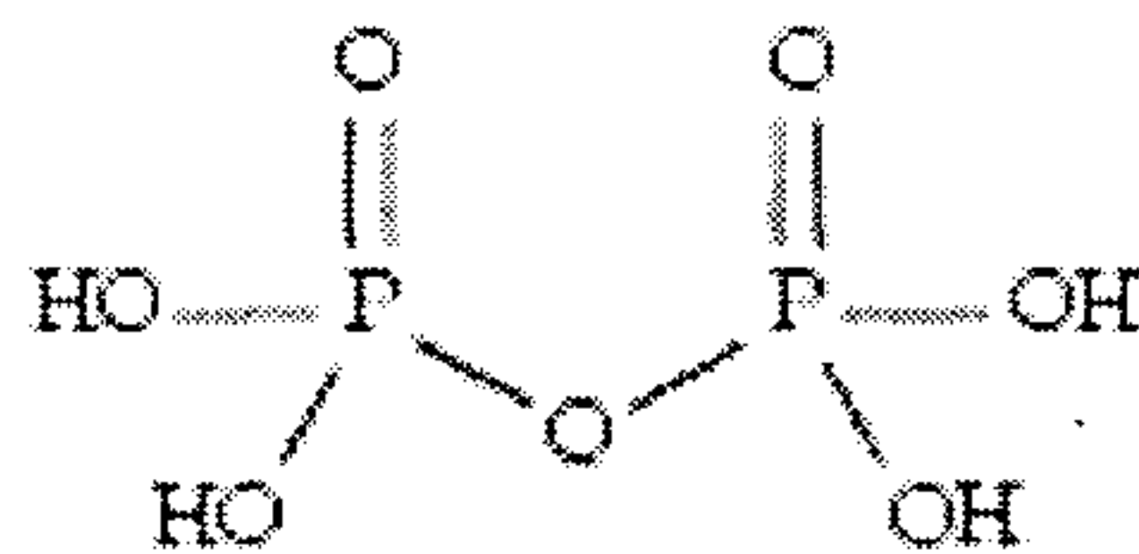
Pyrophosphoric acid
