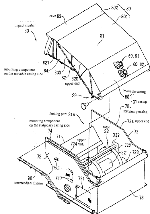
Figure 6 Exploded Perspective View of the Crusher
